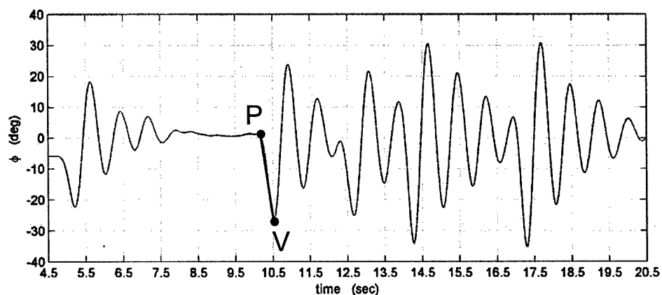
Figure 2-7: Illustration Of FTR FOM [9]
