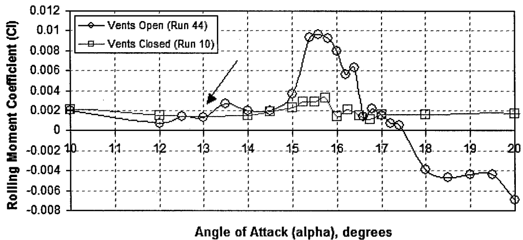
Figure 3-13: Time-Averaged Static Rolling Moment, Static Data
