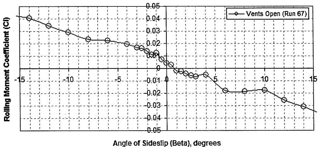
Figure 3-18: Static Lateral Stability for Angle of Attack 15°, Static Data.
