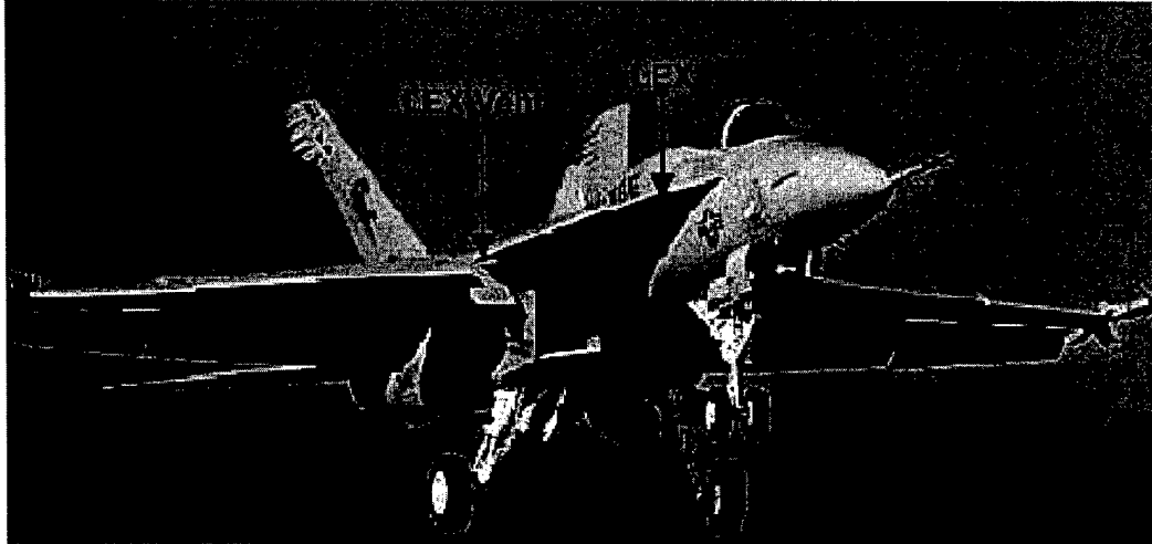
Figure 1-2: Pre-production F/A-18E/F with LEX Vents in the Open Position [3]
