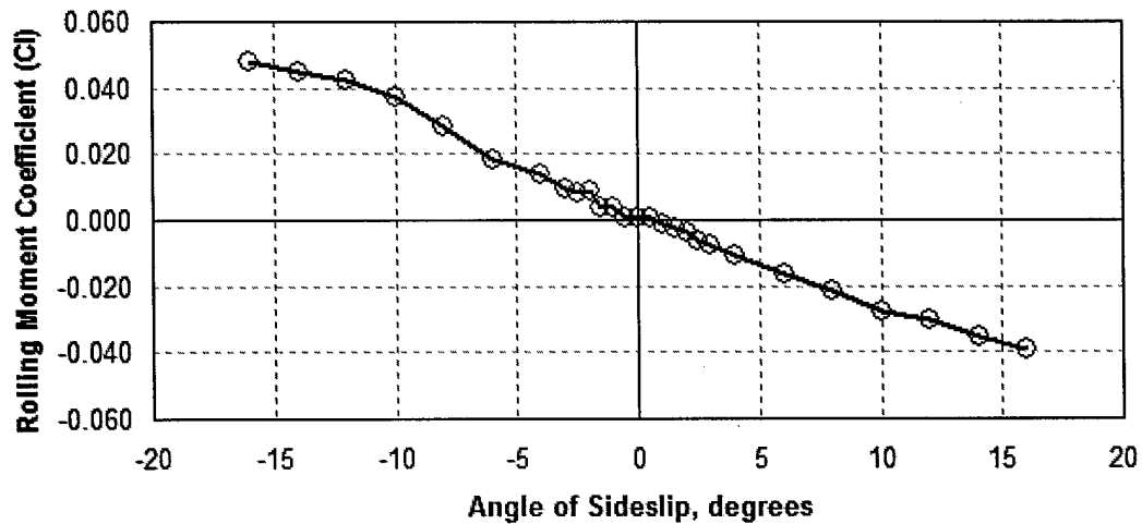
Figure 3-15: Static Lateral Stability for Vents Open Configuration, Angle of Attack 13°, Static Data
