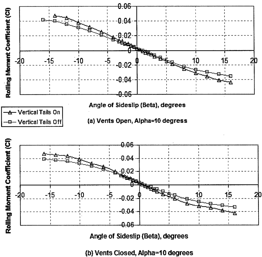
Figure 3-1 (a, b): Effect of Vertical Tail at Angle of Attack 10^\circ
