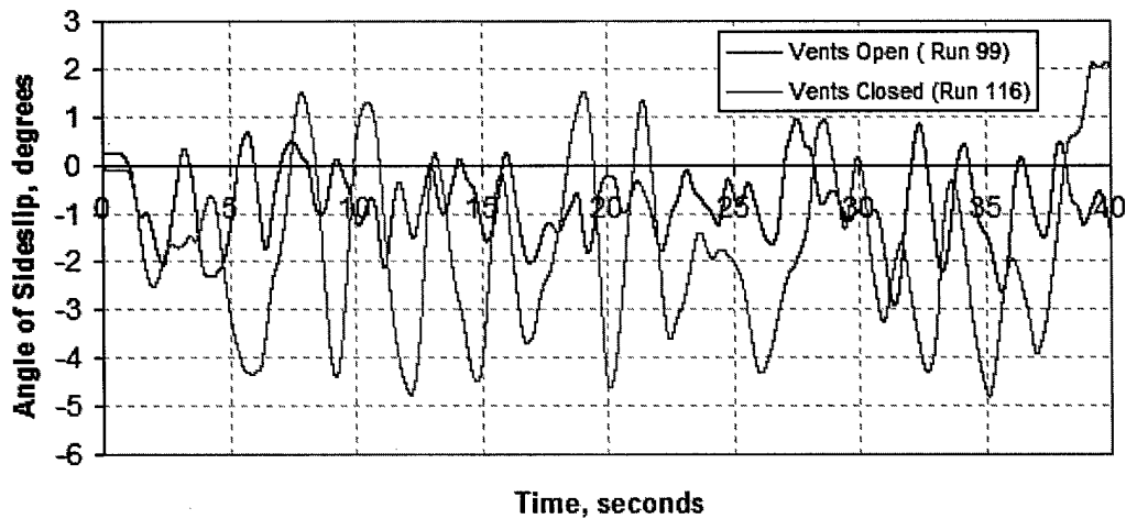
Figure 3-23: Angle of Sideslip Time History for Angle of Attack 16°, FTR Data
