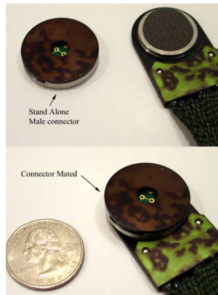
Figure 4. Universal snap fastener
