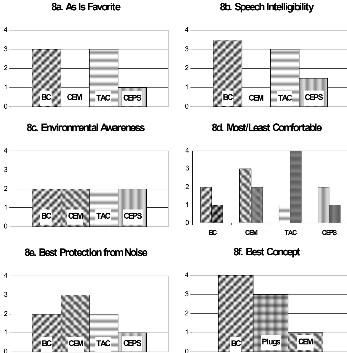
Figure 8. Questionnaire results.
