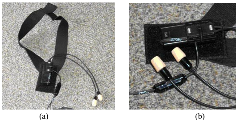
Figure 4. CEPS system: (a) "hook and loop" yoke with interface box and earplugs, (b) close view of interface box and earplugs.
