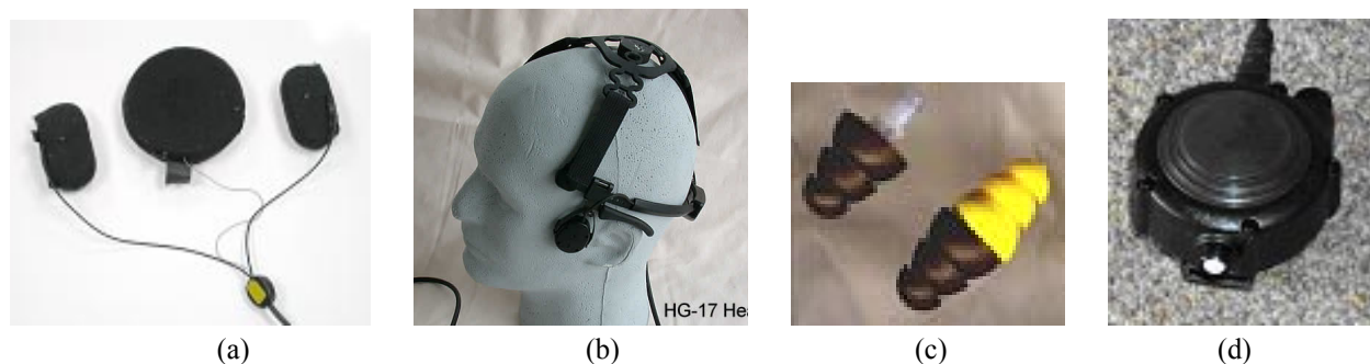
Figure 1. Components of BC configuration: (a) Temco bone conduction contact microphone and vibrators contained in ACH helmet pads, (b) Temco HG-17 webbed headset, (c) CAE showing core with orifices that allow level-dependent hearing protection, and (d) Temco BM-8 push-to-talk button.
