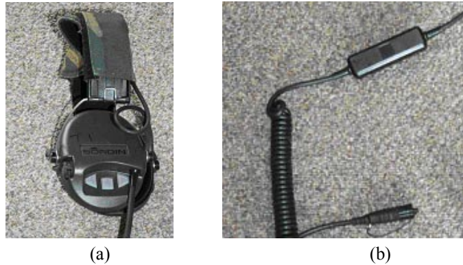
Figure 2. Components of Sordin earmuff system: (a) earmuffs with hear-through microphones and a bone conduction microphone in the ear cup, and (b) push-to-talk button.
