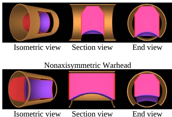
Figure 1: Comparison of conventional axisymmetric warhead with nonaxisymmetric warhead
