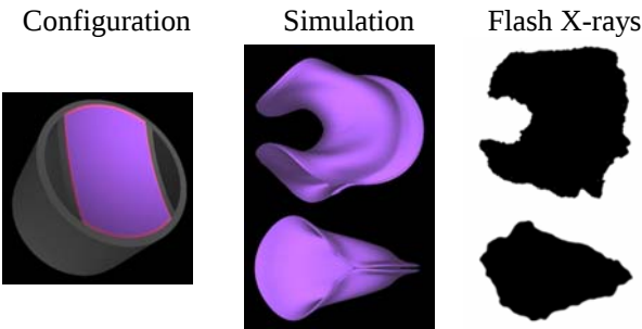
Figure 6: Early nonaxisymmetric warhead test and 3D hydrocode simulation
