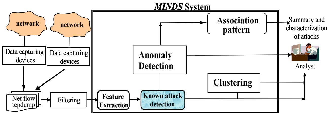
Figure 1 MINDS Architecture
