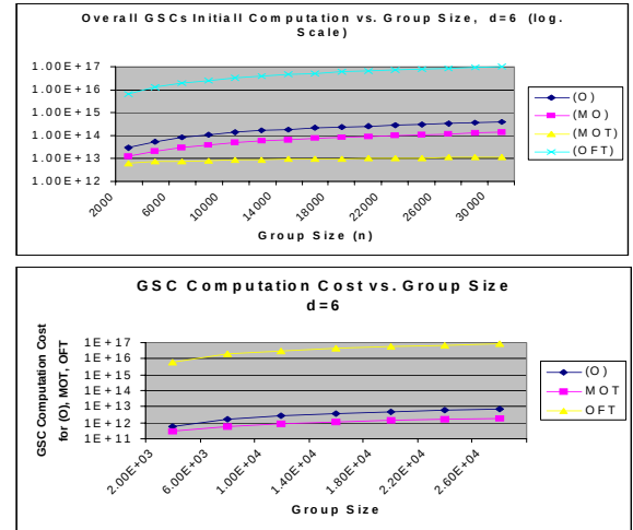
Figures 1, 2: Computation Costs of KM protocols w/o or w/ the consideration for the dynamic CA operation capabilities
