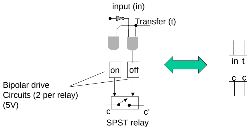
Figure 21. Relay drive circuit.
