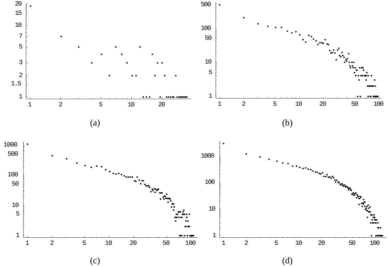
Figure 40. Scale-free distributions produced from nanowire networks. In these plots, x-axis is wirelength, and the y-axis corresponds to the number of wires at particular wirelengths. (a) 20x20 nanowires. (b) 100x100 nanowires. (c) 200x200 nanowires. (d) 400x400 nanowires. ( p_w=p_F=25 nm, \phi=30^\circ , p_C=250 nm, T_{\text{SLAB}}=4 \mu\text{m} , T=1 \mu\text{m} .)
