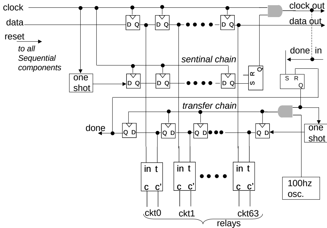
Figure 22. Relay configuration circuit, capable of scaling to multiple sets of relay devices.
