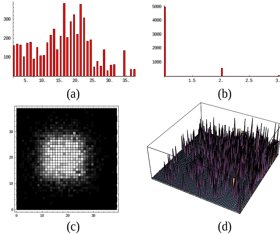
Figure 36. Results of initial nanowire distribution simulation with randomization on wire angles ( p_w=25 nm, p_F=25 \mu m, p_C=250 nm, T=1 \mu m, T_{SLAB}=4 \mu m, \phi=20^\circ , n_{wires} = 14,400 ). Number of nets generated: 5,629, with 673/1,330 unique coarse pads and 5,629 unique fine pad zones. 3,863 nanowires were mapped to fine pads not directly under coarse grid pads.
