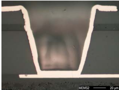
Figure 18. Example of 125μ deep via formed in HDI process (compared to 37μ for standard vias) to contact micro-relay die bond pad to metal level one package metallization in test structure.
