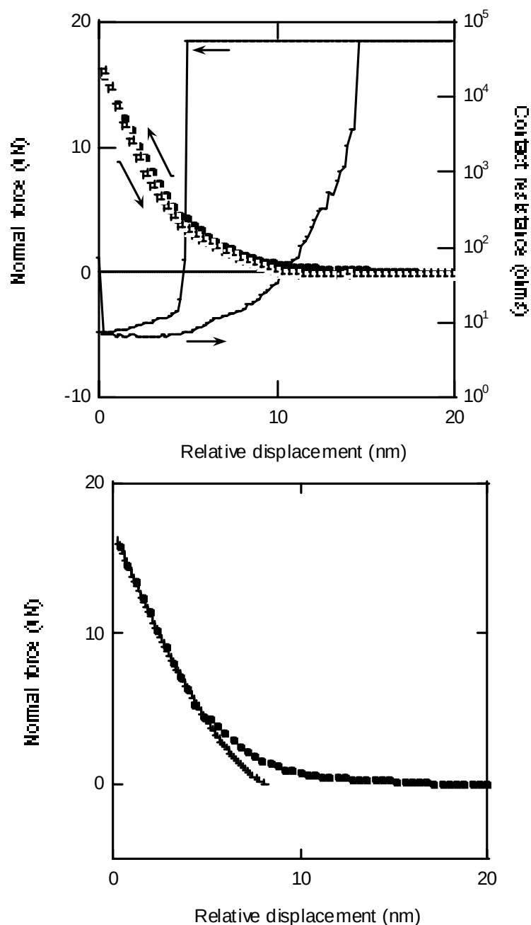
Figure 28. (a) A low-resistance 0.01 mA contact event following tip and substrate ozonation; the minimum contact resistance is about 9 \Omega , achieved after a repulsive breakdown force of \sim 5 \mu N is applied. (b) JKR analysis of the force profile indicates an elastic modulus of 20 GPa
