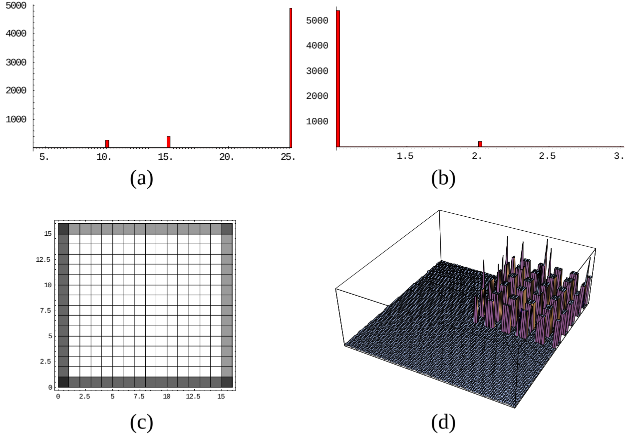
Figure 38. Nanowire distribution simulation without randomization ( p_w=25 \mu\text{m} , p_F=25 \text{ nm} , p_C=250 \text{ nm} , T = 1 \mu\text{m} , T_{\text{SLAB}} = 4 \mu\text{m} , \phi=0.05 , n_{\text{wires}}=14,400 ). Number of nets generated: 5,625. No nanowires were mapped to finepads unless directly under coarse grid pads.
