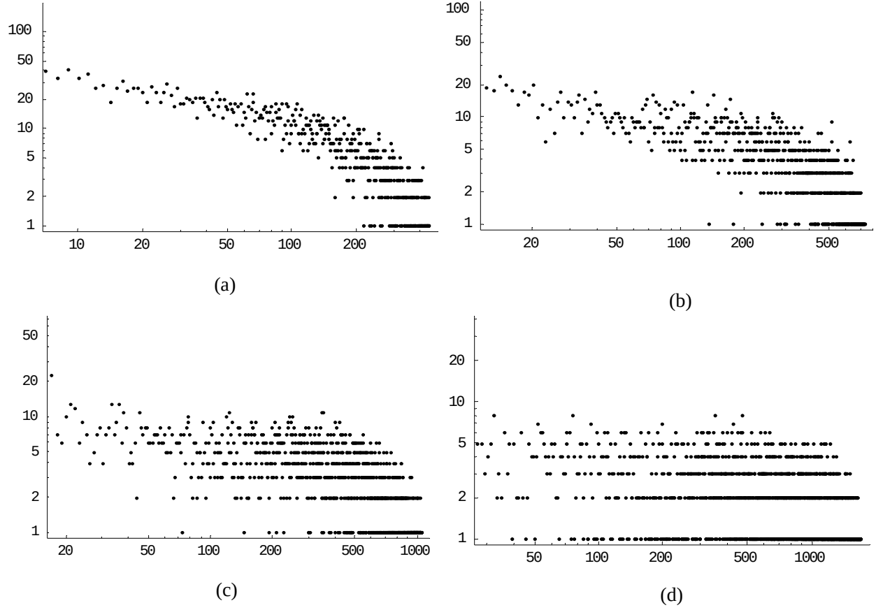
Figure 42. Effects of coning angle on wirelength distribution (concluded). (a) \phi = 65^\circ . (b) \phi = 70^\circ . (c) \phi = 80^\circ . (d) \phi = 85^\circ . ( p_w = p_F = 25 nm, p_C = 250 nm, T_{SLAB} = 4 \mu m, T = 1 \mu m, n_{WIRES} = 14,400 ).
