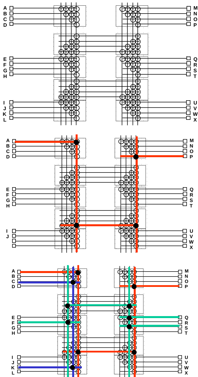
Figure 13. This symbolic representation (top) of the adaptive manifold contains 24 external terminals (A-X), ten small switchboxes, 100 switches, represented. The connection of two or more terminals is accomplished through switch closures. The first example (middle) demonstrates the formation of a net between "A" and "P". The second example (bottom) shows the formation of a network containing nets "AP", "CK", and "FQS".
