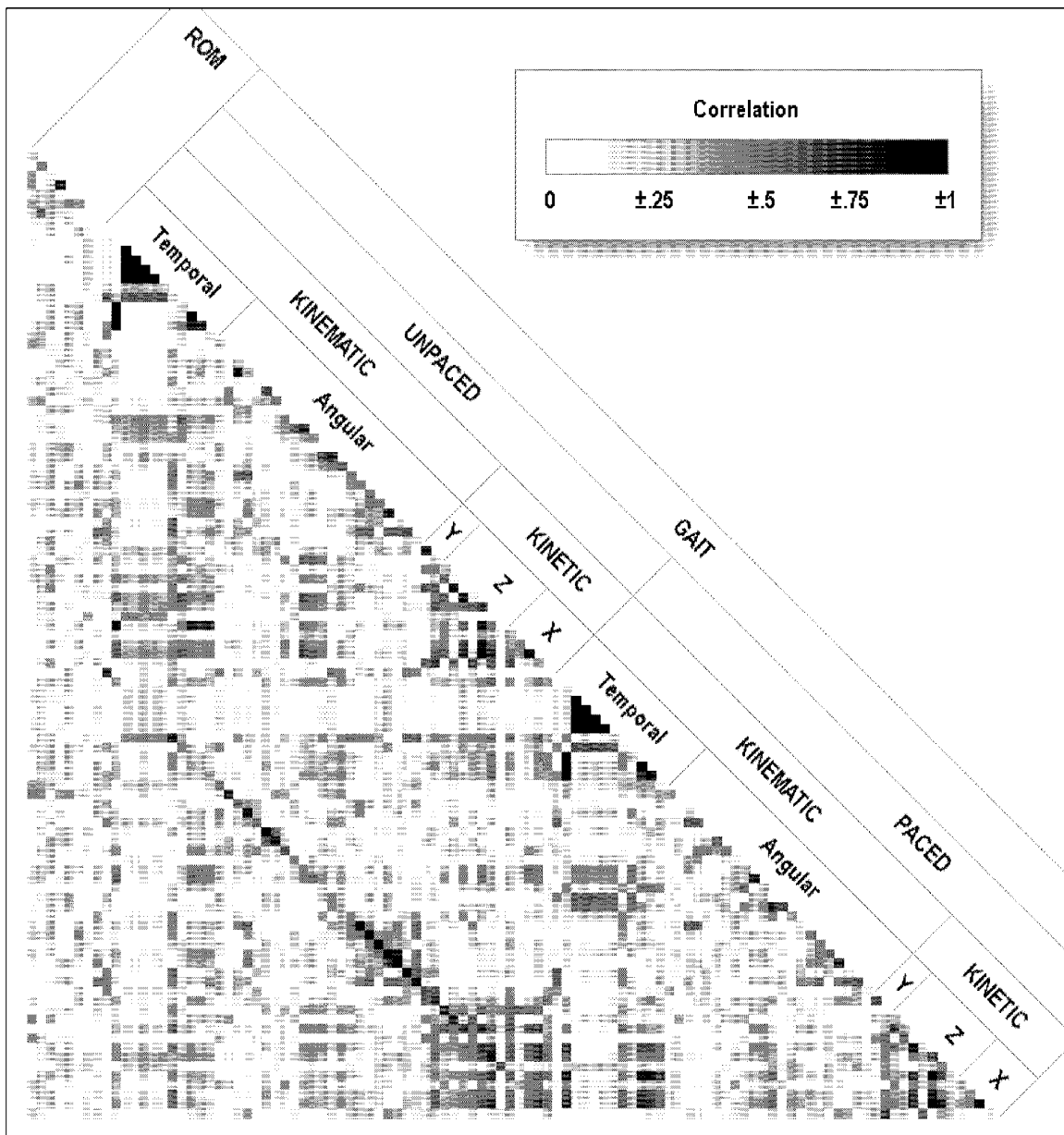
Figure 2. Correlational matrix of the 104 dependent variables. Absolute magnitudes of r are depicted. (See text for further description.)
