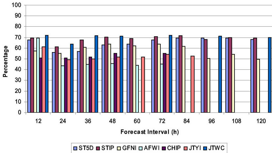
Figure 4.9 Percentage of Good intensity trends as defined in Fig. 4.5 during intensification for the combined 2003 and 2004 seasons. Sample sizes of the verified forecasts range from over 600 at 12 h to less than 200 by the 96-h point. A Good forecast during intensification indicates that the magnitude of the forecast intensification rate is within +/- 10 kt of the actual intensification rate.
