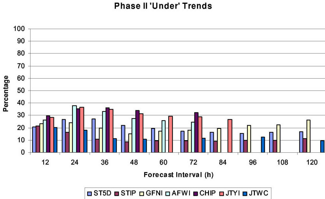
Figure 4.10 Percentage of Under intensity trends as defined in Fig. 4.5 during intensification for the combined 2003 and 2004 seasons. Sample sizes of the verified forecasts range from over 600 at 12 h to less than 200 by the 96-h point. An under-forecast during intensification indicates that the magnitude of the forecast intensification rate is less than the magnitude of the actual intensification rate.
