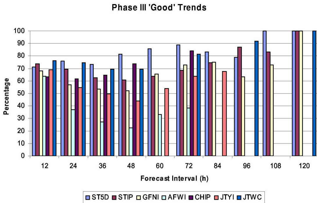
Figure 4.16 Percentage of Good intensity trends during the decay Phase III for the combined 2003 and 2004 seasons. Sample sizes of the verified forecasts range from 400 at 12 h to less than 30 by the 96-h point. A Good forecast during decay indicates that the magnitude of the forecast decay rate is within +/- 10 kt of the actual decay rate.
