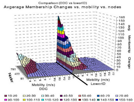
Fig. 1: Average membership changes required from lower ID and DDC algorithms
