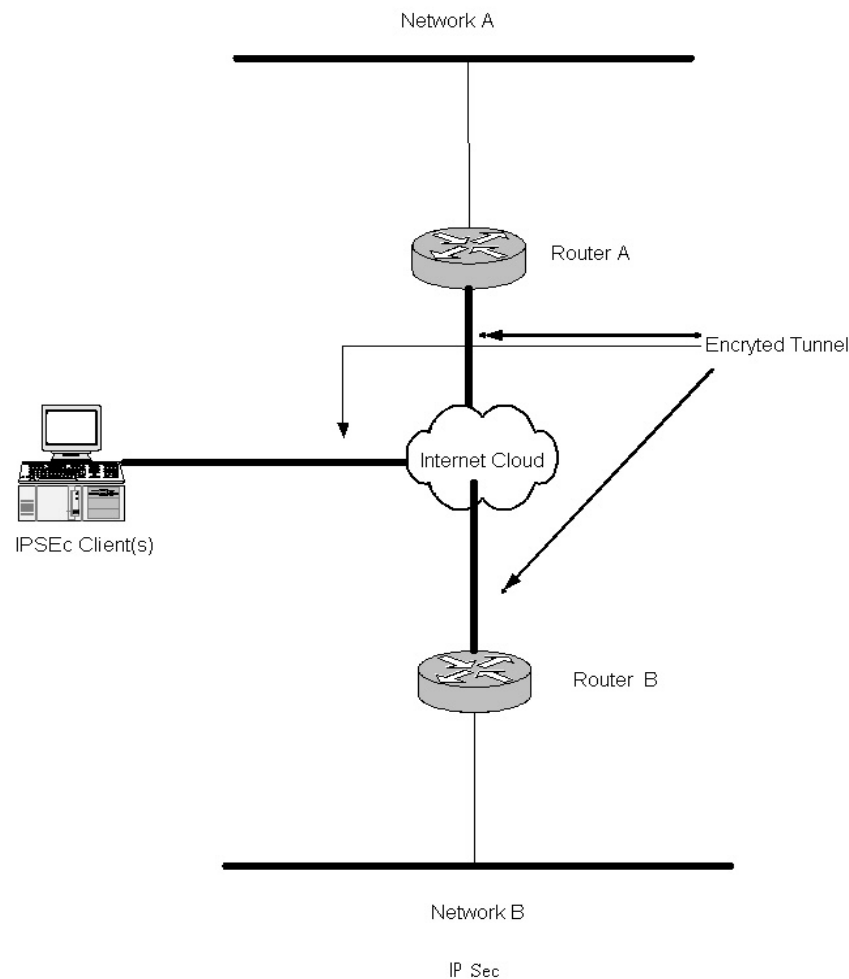
Figure 5: IPsec.
