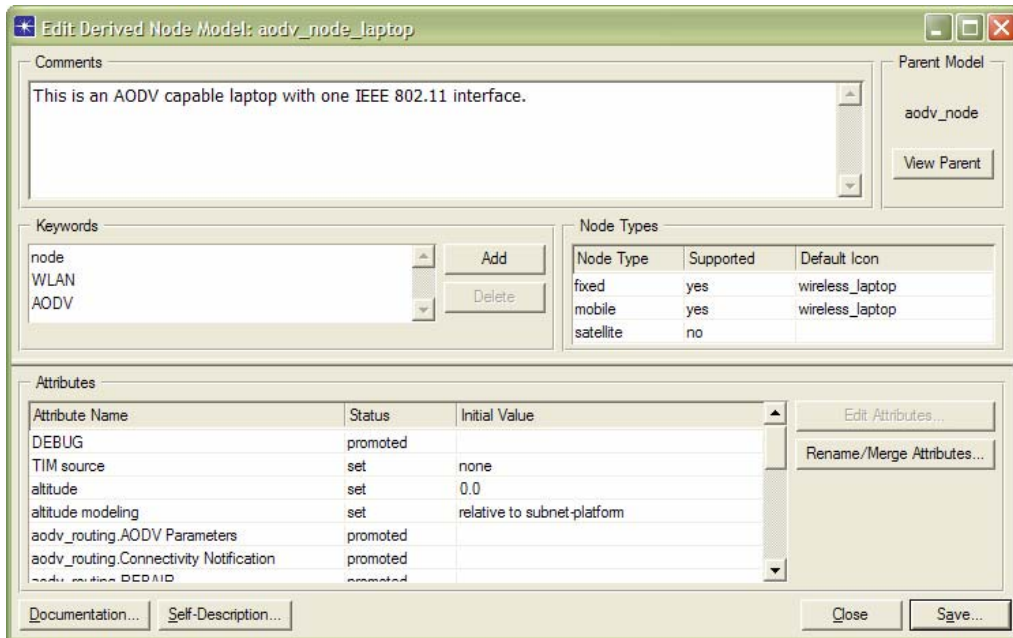
Figure 15. AODV laptop node derivation
