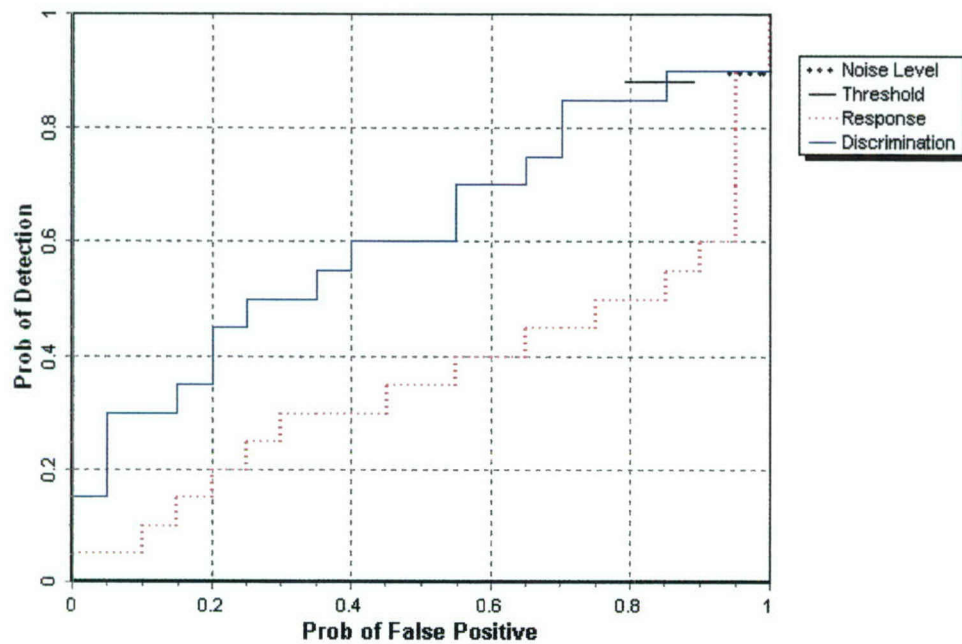
Figure 4. MTADS GEM-3 Blind Grid probability of detection for response and discrimination stages versus the respective probability of false positive for all ordnance larger than 20 mm.
