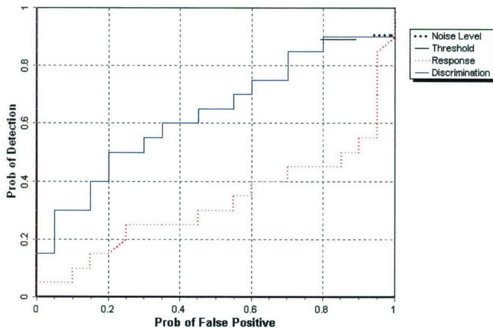
Figure 2. MTADS GEM-3 Blind Grid probability of detection for response and discrimination stages versus the respective probability of false positive over all ordnance categories combined.
