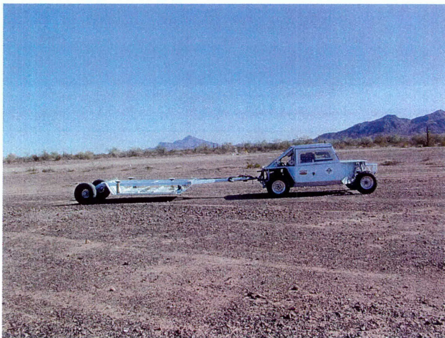
Figure 1. Demonstrator's system, MTADS GEM-3.
