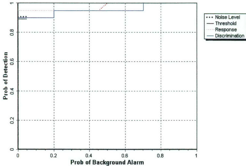
Figure 3. MTADS GEM-3 Blind Grid probability of detection for response and discrimination stages versus the respective probability of background alarm over all ordnance categories combined.
