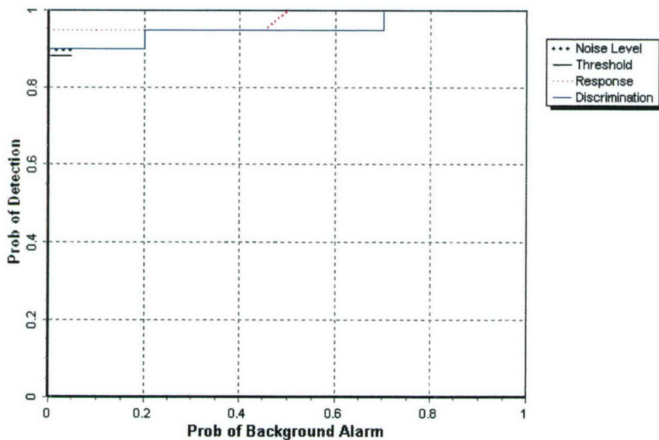
Figure 5. MTADS GEM-3 Blind Grid probability of detection for response and discrimination stages versus the respective probabilities of background alarm for all ordnance larger than 20 mm.
