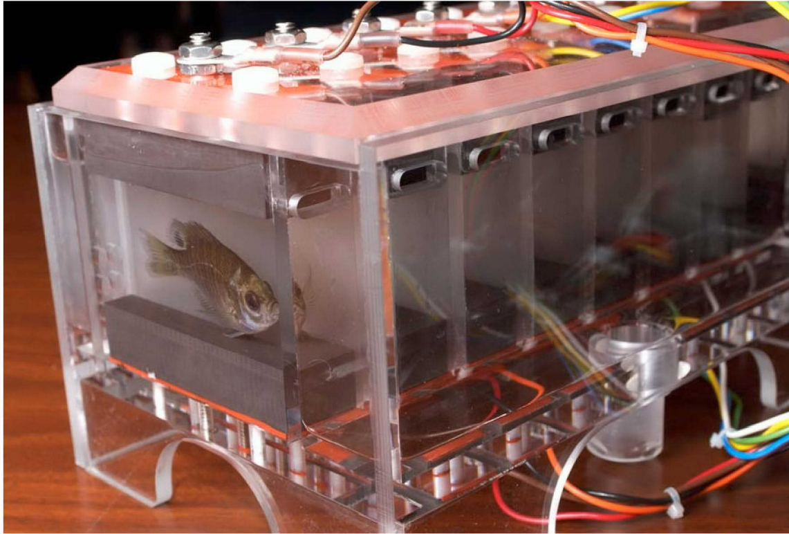
Figure 1. Aquatic Biomonitor Chamber. The chamber contains eight cells, with one fish in each cell. Ventilatory and movement patterns are monitored using the carbon block electrodes above and below each fish.
