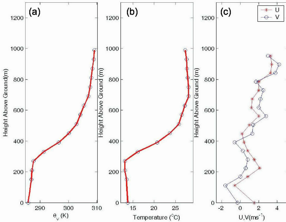
Figure 5. Vertical profiles of the lower atmosphere from the profiler/RASS measurements. (a) Virtual potential temperature, \theta_v ; (b) virtual temperature directly from the RASS measurements; and (c) Horizontal wind components.
