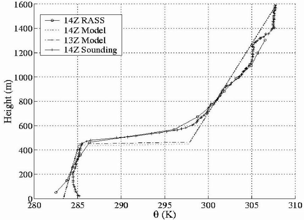
Figure 23. Comparison of model initial conditions
