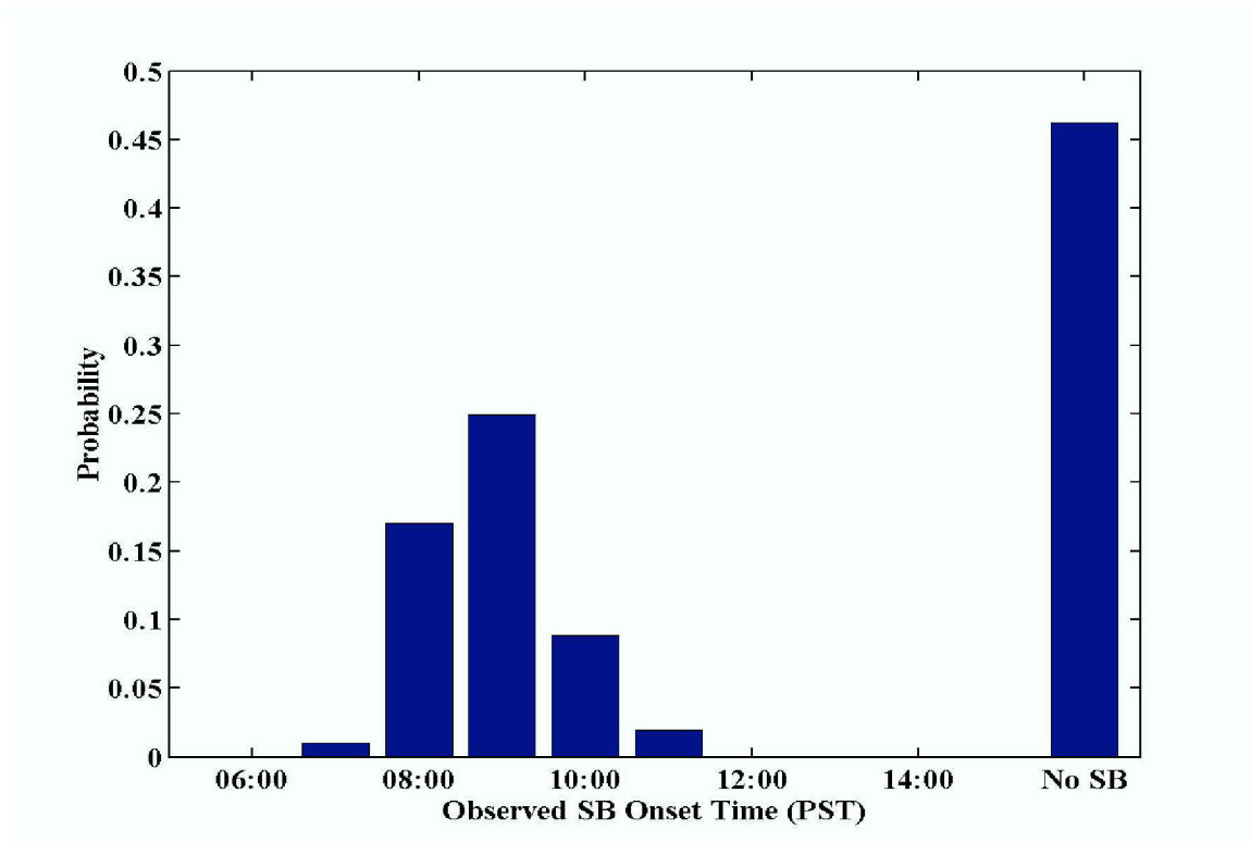
Figure 21. Frequency of occurrence (or probability) of the beginning of SB onset. The non-sea breeze condition (No SB) is listed as a separate category.
