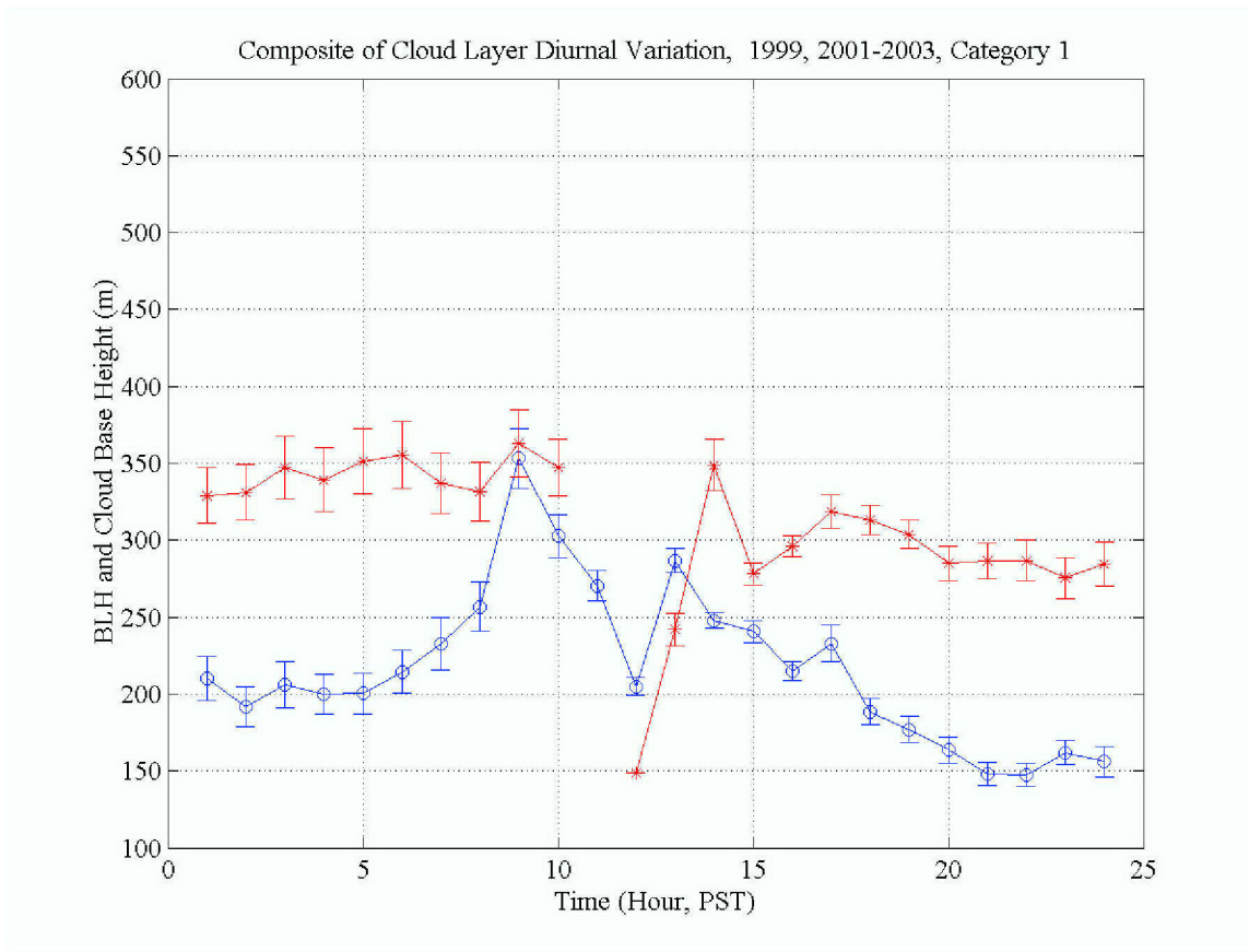
Figure 12. Composite BLH and cloud base height for Category 1 cases. The red line shows the boundary layer top obtained from profiler/RASS profiles; the blue line shows the cloud base height from the CT25K ceilometer. The vertical bars denote the range of the 95% confidence interval.
