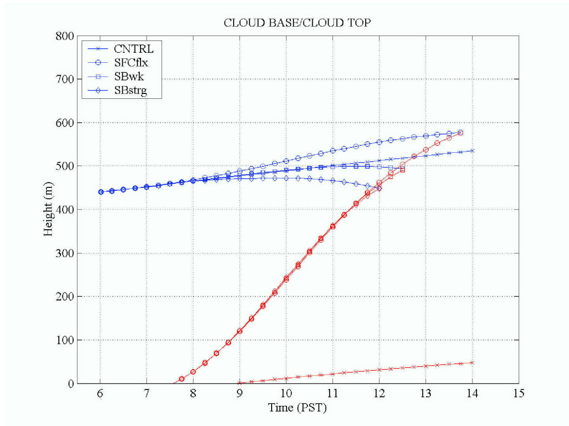
Figure 26. Evolution of cloud base and cloud top height for all four simulated cases.
