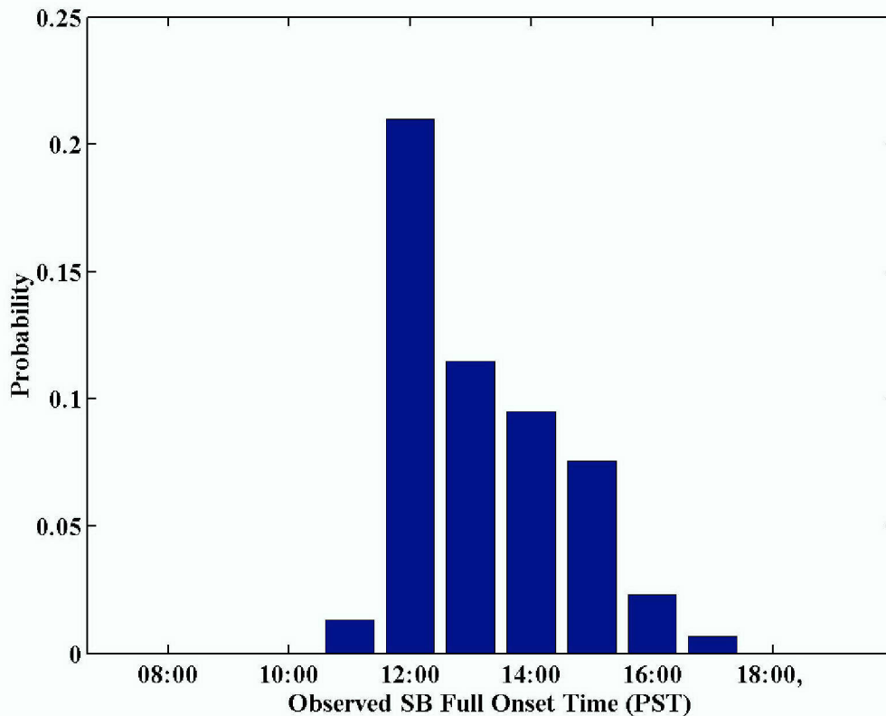
Figure 22. Same as in Figure 21, except for the SB full development time
