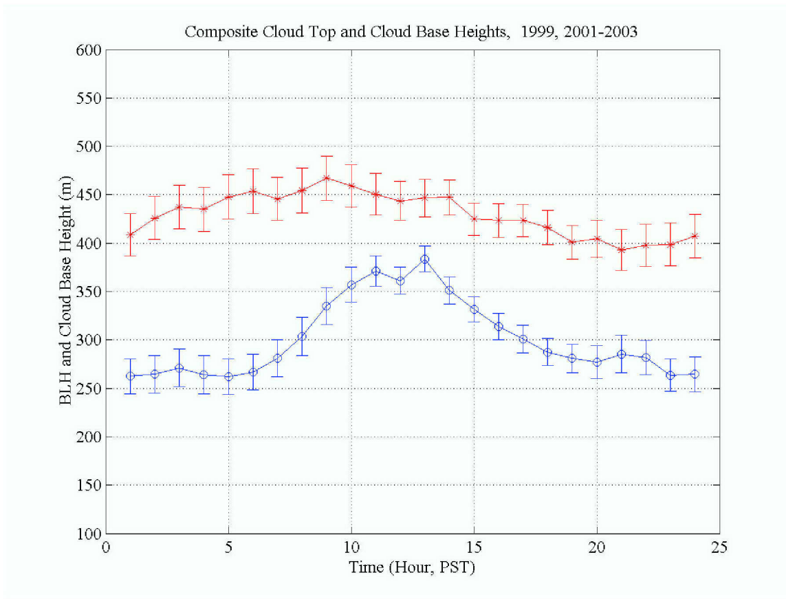
Figure 18. Same as Figure 12, except for all 10-summer months of data used in this study.
