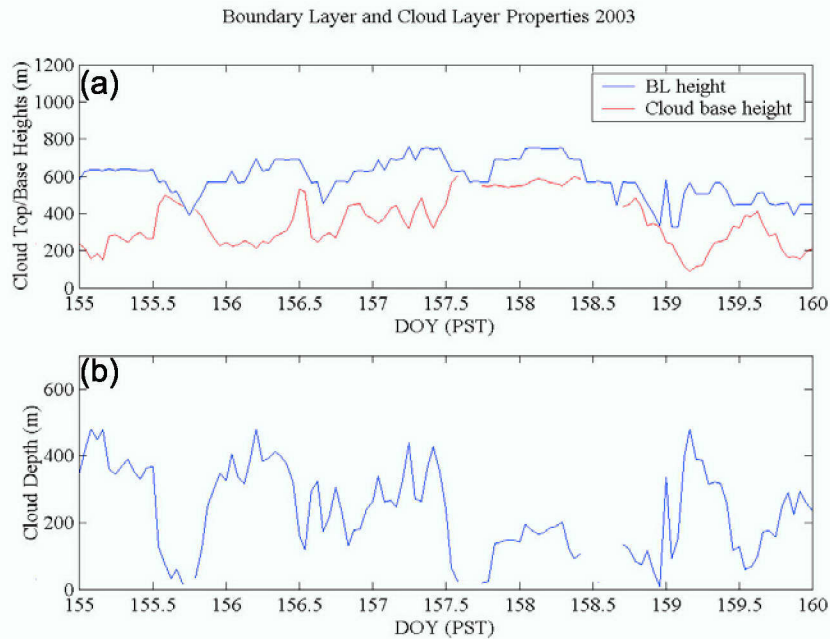
Figure 10. Diurnal variation of (a) BLH and cloud base height (m); and (b) cloud depth between June 4 and June 9 of 2003.
