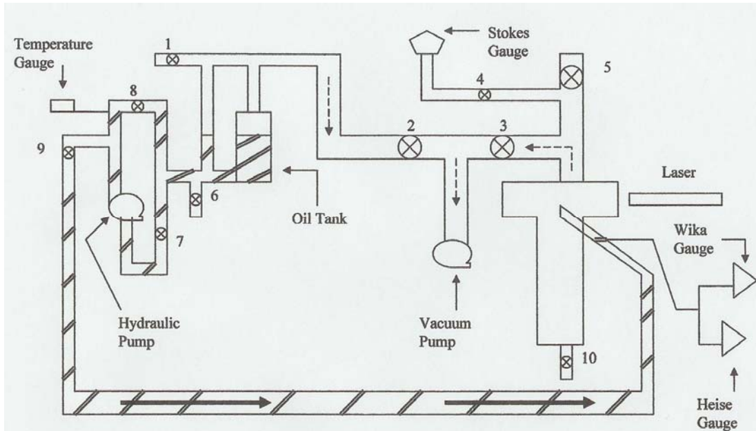
Figure 82. Schematic diagram of vacuum chamber and LDV
