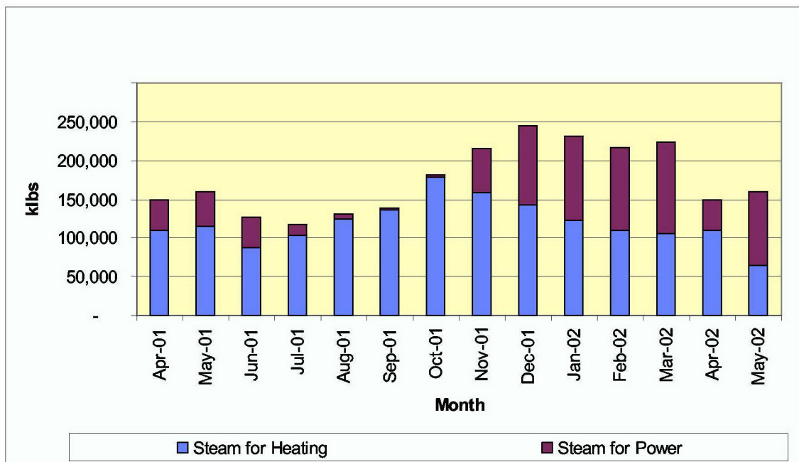
Figure 3. FWA monthly steam usage for heat and power.
