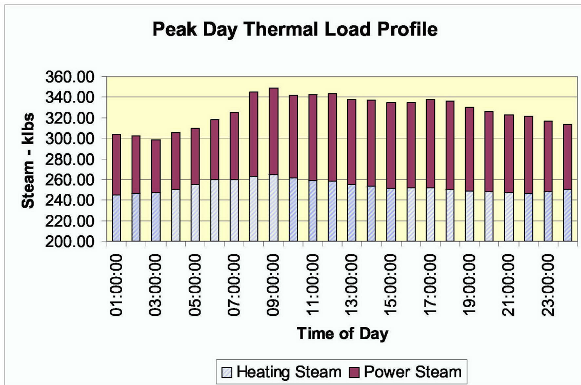
Figure 6. Thermal load profile during peak demand day, 6 November 2001.
