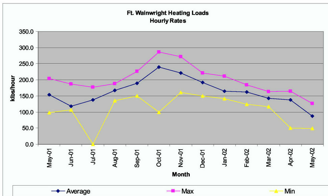
Figure 4. FWA hourly steam requirements for heat.
