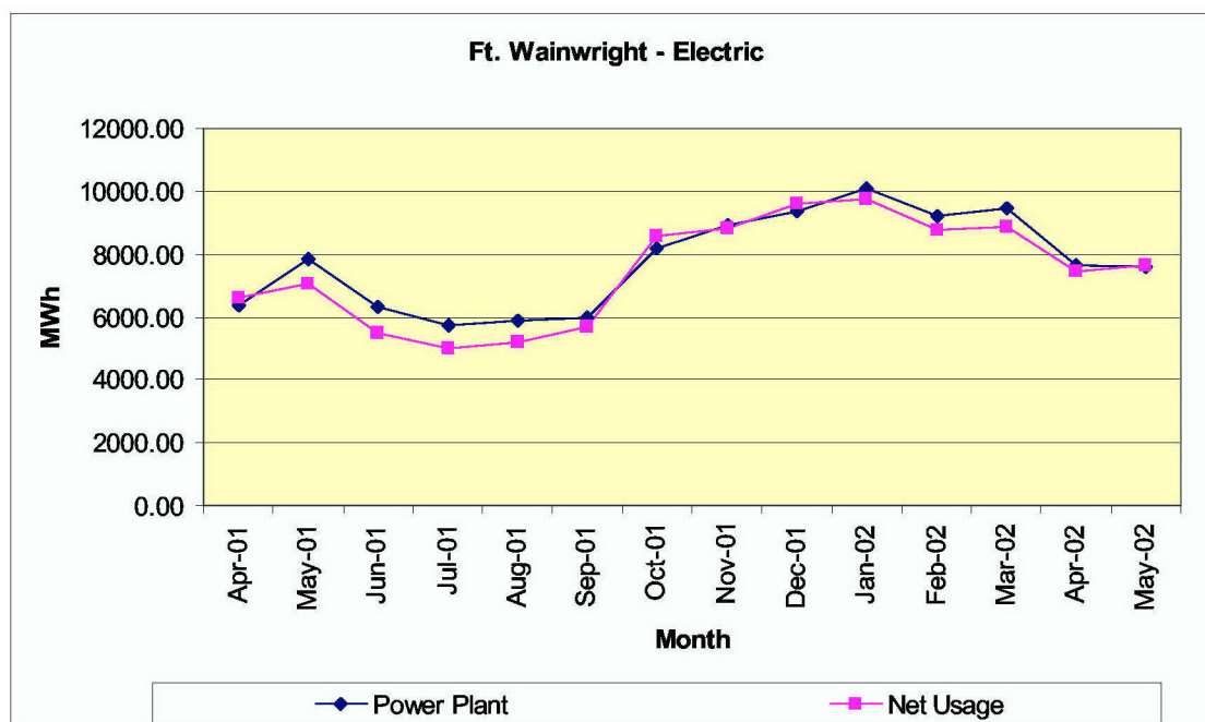
Figure 2. FWA's CHPP monthly totals of electrical generation, and the net electric usage for FWA.
