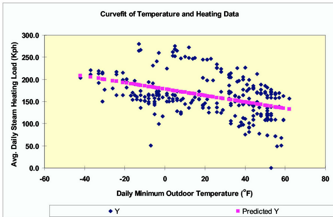
Figure 9. Regression line for the steam heating load (Kph) vs. outdoor ambient temperature (°F).
