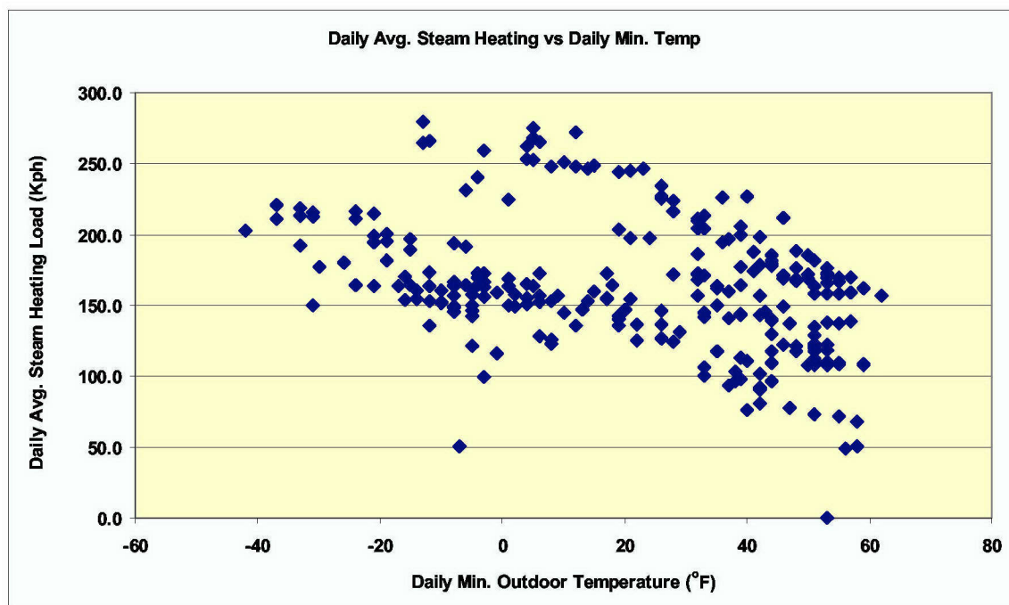
Figure 8. Steam heating load (Kph) vs. outdoor ambient temperature (°F).
