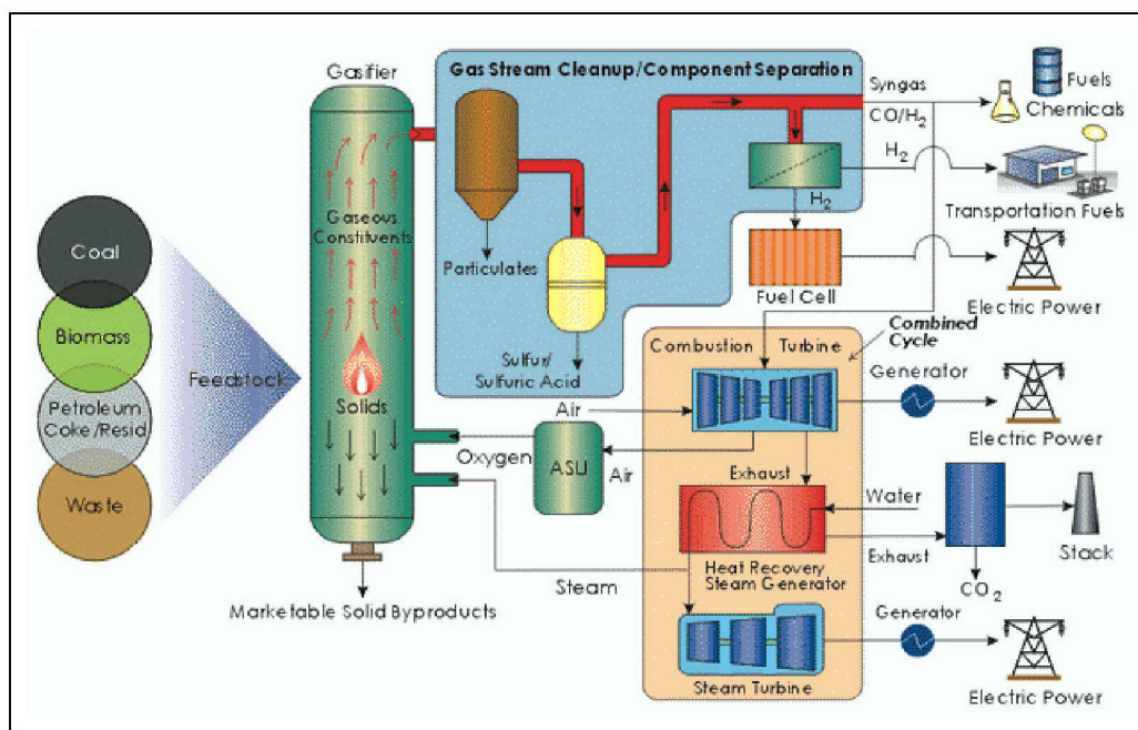
Figure 11. Schematic of coal gasification.
