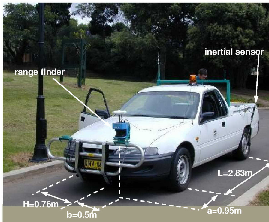
Figure 7: Vehicle Geometry
