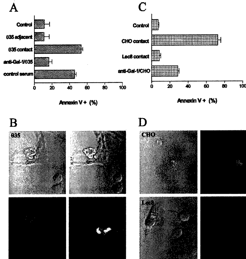
FIG. 1. Galectin-1 on the stromal cell surface kills adherent T cells. A and B, Pha R 2.1 T cells were added to subconfluent monolayers of 035 thymic stromal cells for 1 h. Cell death was assessed by annexin V-FITC binding. The % annexin V + T cells in contact with or adjacent to 035 cells was determined for 50–100 T cells in 5–8 microscopic fields. The top bar in A indicates % annexin V + T cells in the absence of 035 cells. Death was inhibited by the addition of anti-galectin-1 antiserum (anti-Gal-1). Panel B is a phase image of an adherent 035 cell and a T cell (upper left), annexin V-FITC staining of the T cell (lower left), overlay of the phase and fluorescent images (upper right), and galectin-1 expression by a 035 cell (red) and annexin V-FITC binding by an adherent T cell (green) (lower right). C and D, Pha R 2.1 T cell death was assessed as above on CHO or Lec8 cells. The top bar in C indicates the percent annexin V + T cells in the absence of CHO or Lec8 cells. Panel D shows phase images of T cells bound to CHO and Lec8 cells; numerous annexin V + T cells were bound to CHO cells, whereas T cells bound to Lec8 cells did not become annexin V + . In A and C values are the mean of triplicate samples in a representative experiment.
