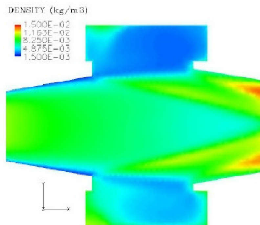
Figure 7 Closeup density contours in test section
