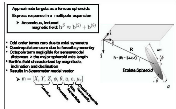
Fig. 4. Example of parametric model to simulate the induced TFM response of an axisymmetric target (prolate spheroid).
