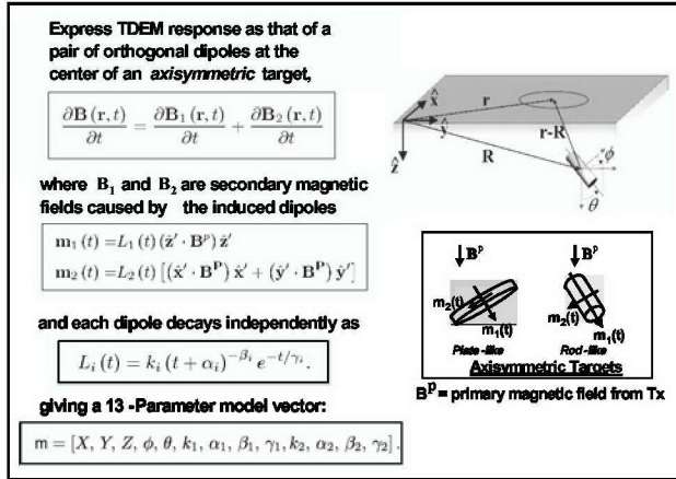
Fig. 5. Example of parametric model to simulate the TDEM response of an axisymmetric target.
