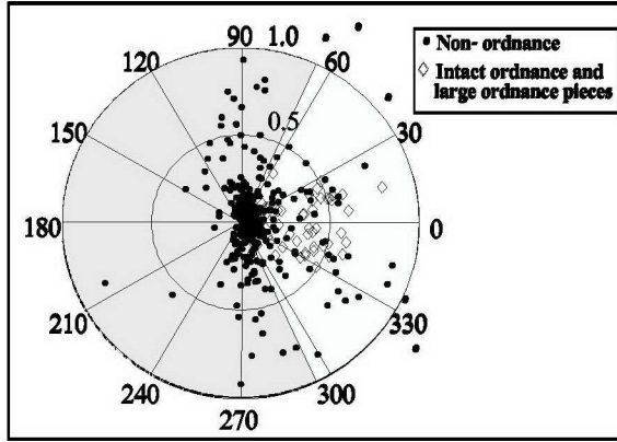
Fig. 9. Recovered dipoles from a TFM survey at a Montana site, keyed to the results of excavating all 822 identified targets
