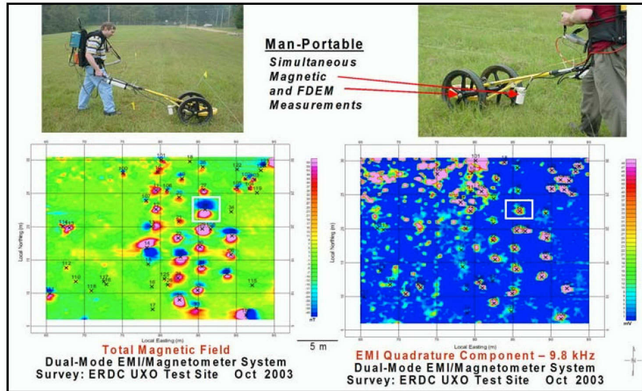
Fig. 12. New dual-sensor system (FDEM and TFM). Datasets acquired with new system at the ERDC UXO Test Site, Vicksburg, MS.
