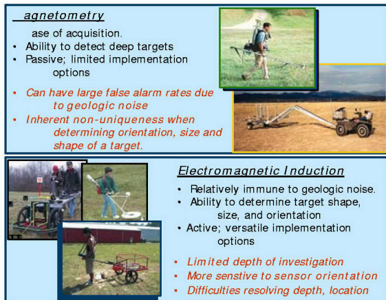
Fig. 2. Advantages and limitations of magnetometry (TFM) and electromagnetic induction (EMI).
