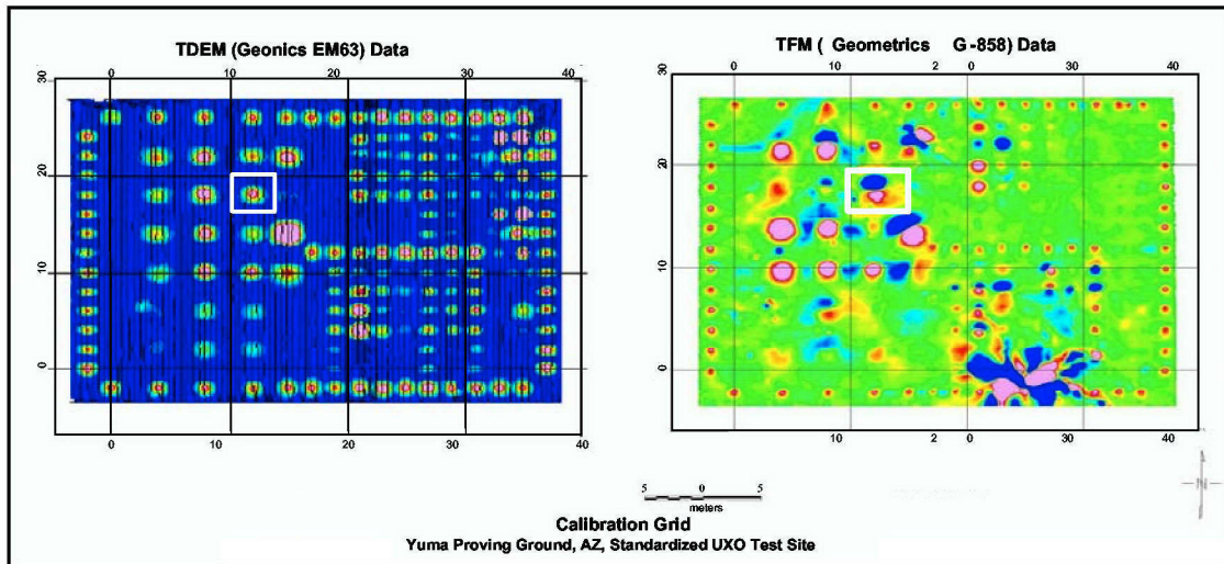
Fig. 13. TDEM (left) and TFM (right) datasets acquired on the Calibration Grid of a Standardized UXO Test Site. Each 1- × 1-m “cell” in the Calibration Grid is either empty or contains a known buried target; the known targets are either inert ordnance items or standard objects such as plates or solid spheres.
