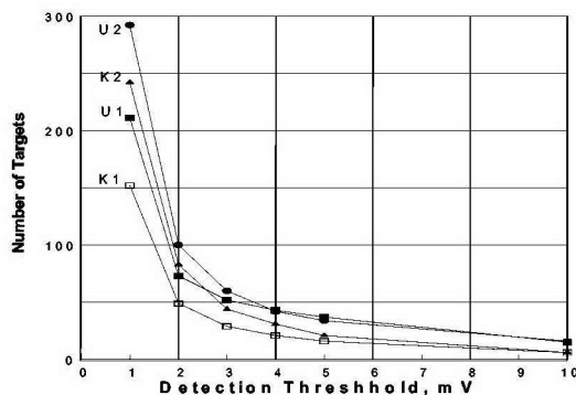
Fig. 3. Number of targets vs. detection threshold for TDEM surveys of four seeded test sites at Former Fort Ord, California.
