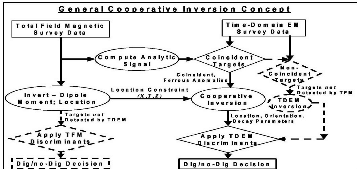
Figure 11. Concept of a process flow and general cooperative inversion algorithm, where the target location, obtained from inversion of TFM data, is constrained during inversion of the corresponding TDEM data. The processing flow allows for (1) discrimination using a location constraint during the TDEM inversion and the TDEM discriminants for targets detected by both methods, (2) discrimination using the TFM discriminants for targets detected only by TFM, and (3) using the TDEM discriminants for targets detected only by TDEM.
