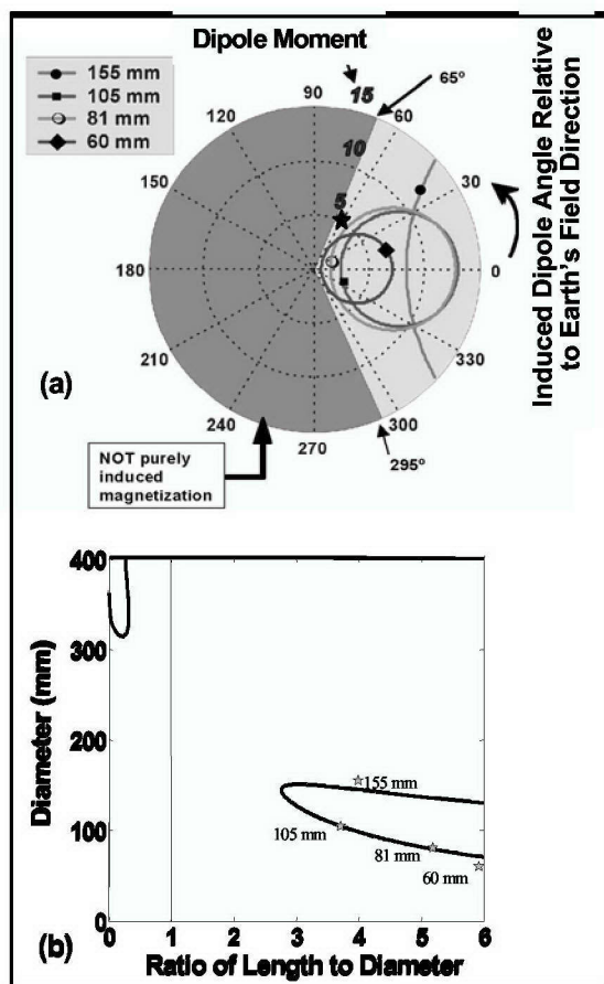
Fig. 8. Illustration of the non-unique magnetic dipole signatures of ordnance models: (a.) different sized spheroids can produce the same dipole moment; the angle of the induced dipole moment relative to the Earth's field direction is limited to < 65^\circ for purely induced magnetization; (b.) spheroid dimensions giving the same dipole moment as 105-mm projectile at 45 deg to Earth's field.
