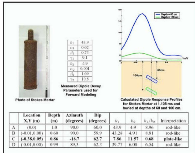
Fig. 10. Example of forward modeling to predict signatures of a stokes mortar. Imposing a TDEM noise floor 0.5 mV, the table of inversion results indicates correct location and orientation recovery and classification for the 60-cm depth case (B), misclassification of the 100-cm depth case (C), and greatly improved location and orientation recovery and correct classification for the 100-cm depth case with a +/- 5-cm location constraint (D). Entry A is the correct location, orientation, and classification.
