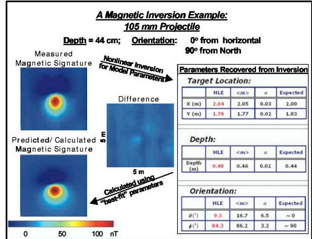
Fig. 6. Illustration of inversion of measured TFM data for model parameters (Fig. 4), where MLE is the maximum likelihood estimate of the parameters and <m> is the mean value of all estimates (Billings et al. 2002)
