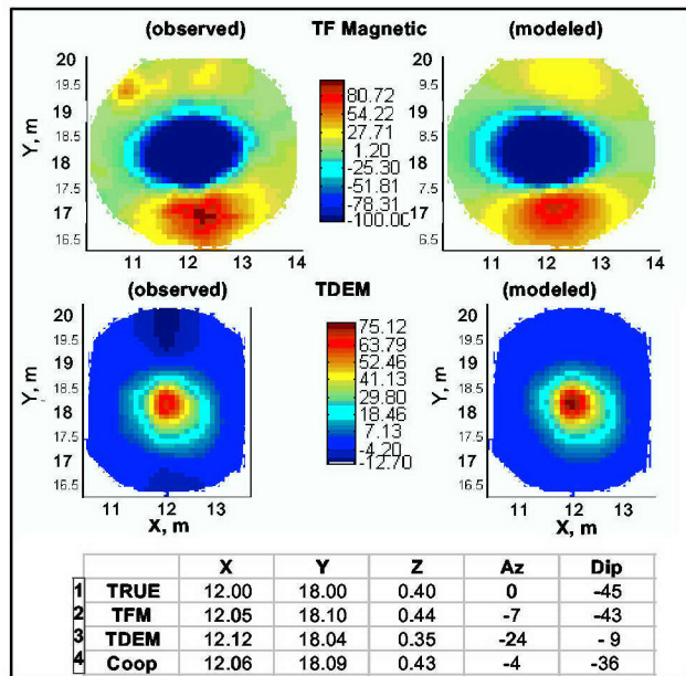
Fig. 14. Observed and modeled (using parameters recovered from inversion) TFM (top) and TDEM (middle) data panels (maps). Table compares known (true), TFM inversion results, TDEM inversion results, and the cooperative inversion results.
