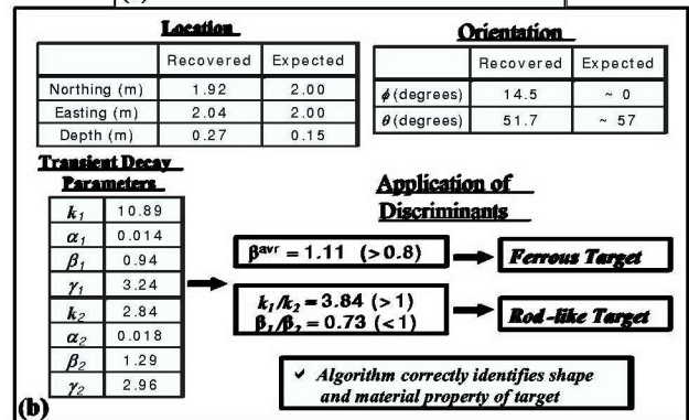
Fig. 7. Illustration of inversion of measured TDEM data over a 60-mm mortar using the model shown in Fig. 5: (a) measured and predicted data and the difference for four selected measurement times; (b) recovered model parameters (Pasion and Oldenburg 2001).
