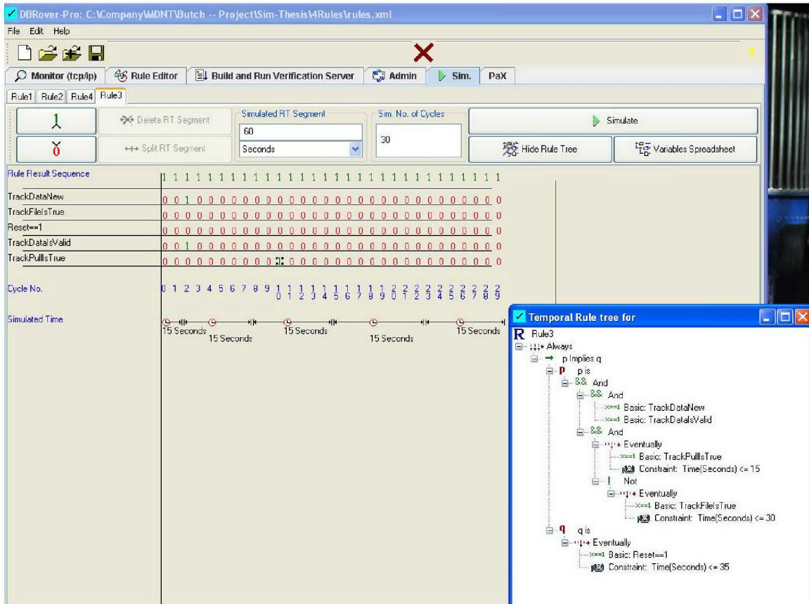
Figure 29. Safety Component: Rule 3, Scenario 4
