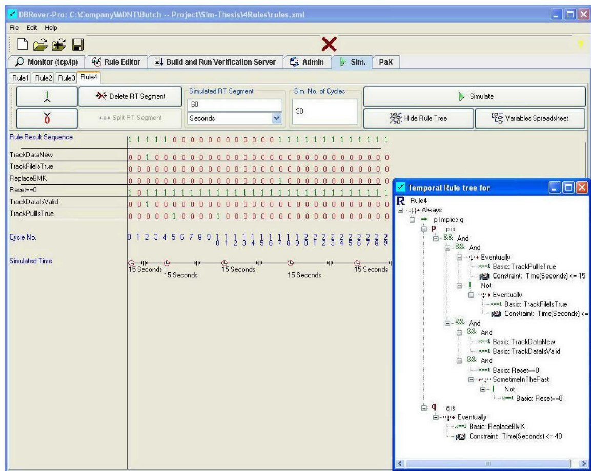
Figure 31. Safety Component: Rule 4, Scenario 2
