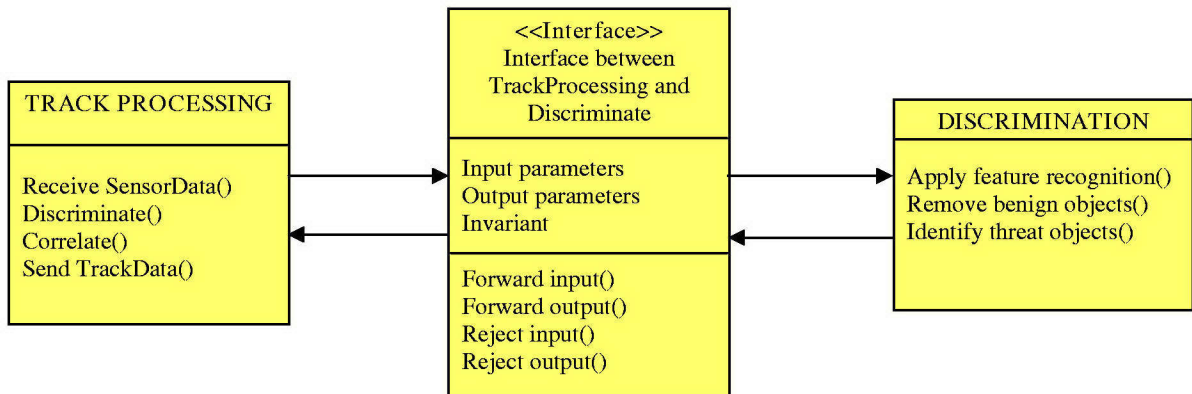
Figure 12. Track Processing Component Interface to Discrimination Component
