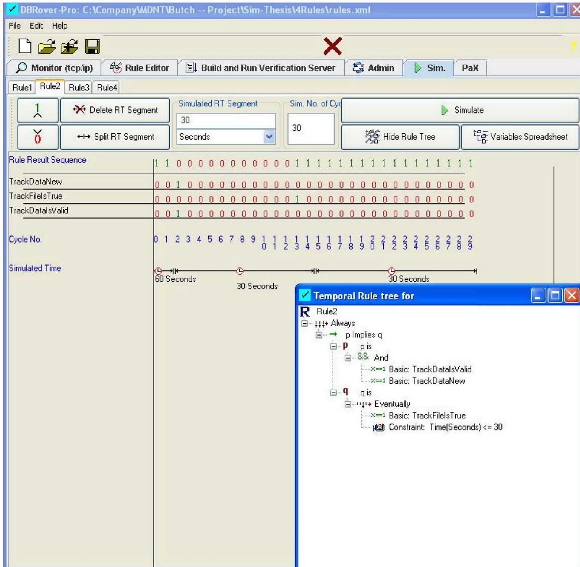
Figure 23. Safety Component: Rule 2, Scenario 1
