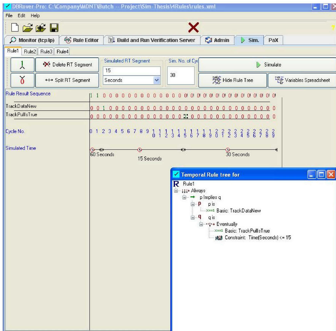
Figure 21. Safety Component: Rule 1, Scenario 2
