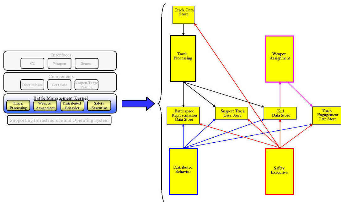
Figure 9. BMK Architecture
