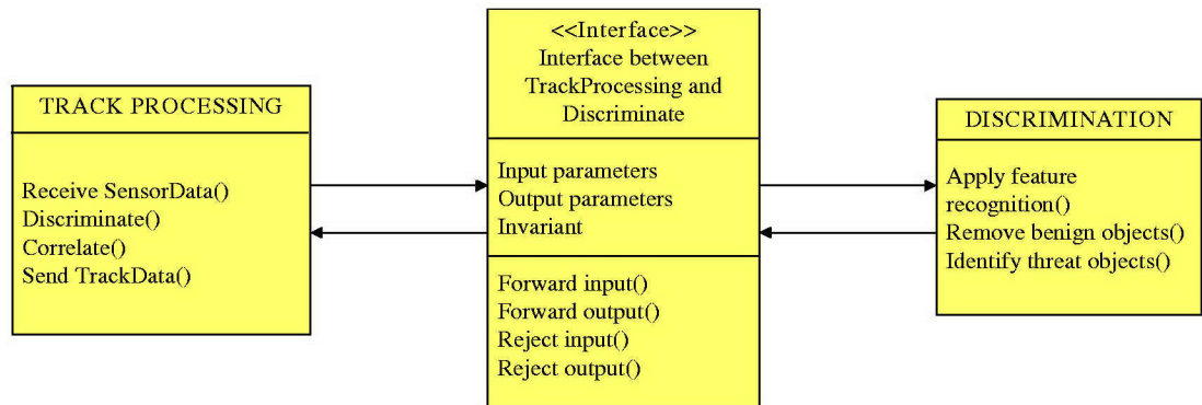
Figure 8. Class Diagram
