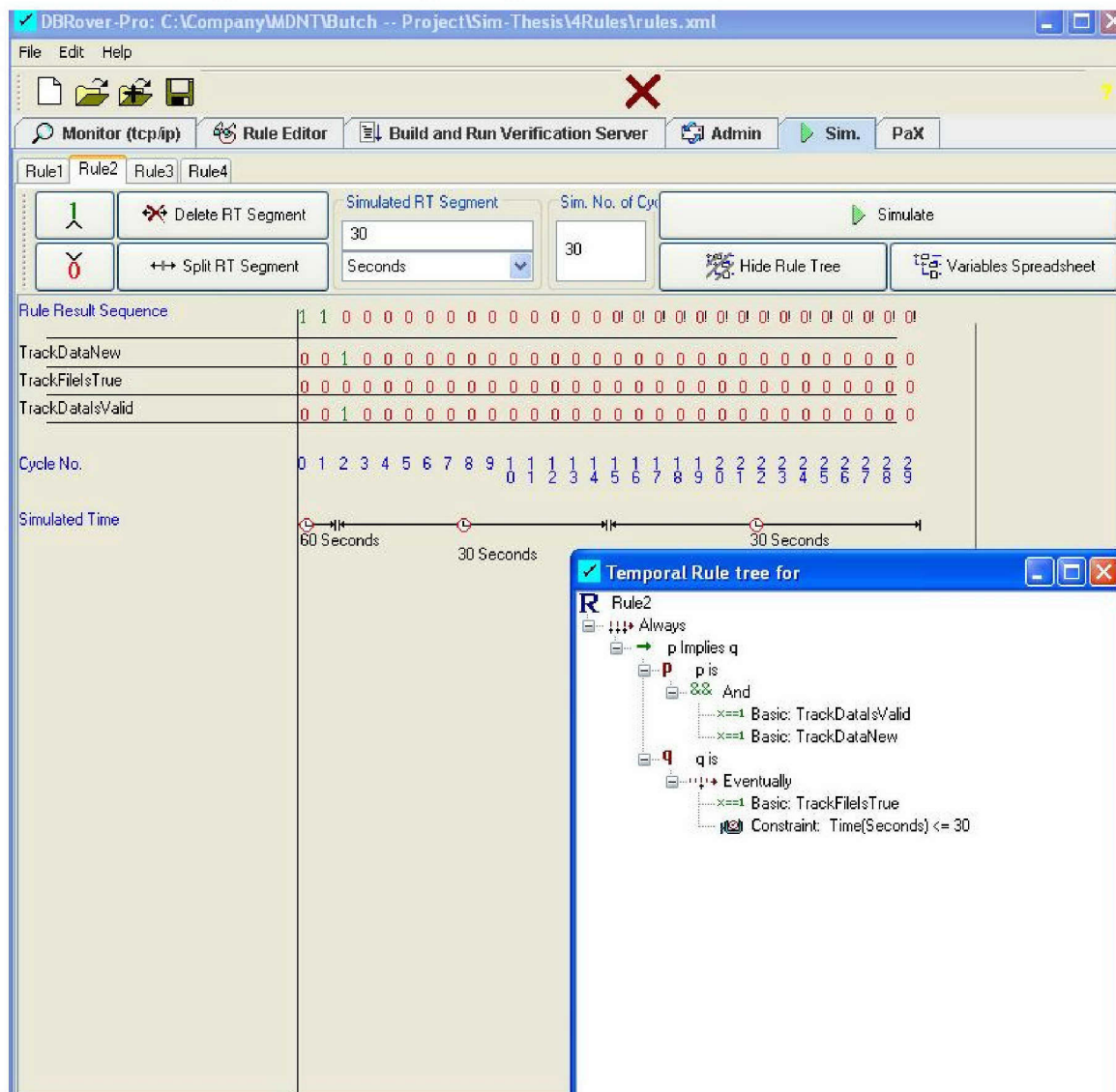
Figure 24. Safety Component: Rule 2, Scenario 2
