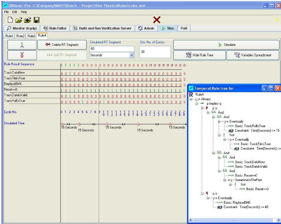
Figure 30. Safety Component: Rule 4, Scenario 1
