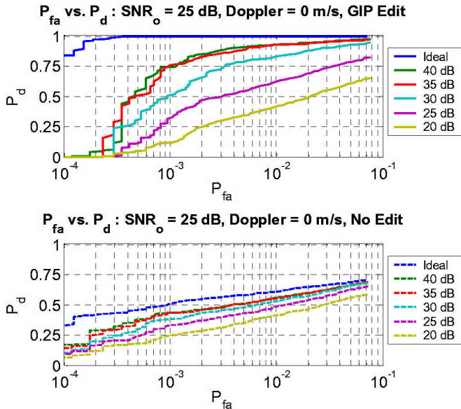
Fig. 5. P_d vs. P_{fa} curves for Doppler velocity 0 m/s with PD5. Unedited and GIP-edited results for all LFM waveforms shown. Legends indicate waveform type/peak sidelobe level.
