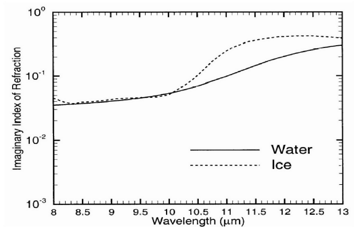
Figure 12. Imaginary index of refraction for water and ice in the 8-13μm window region (from Baum et al 2000).
