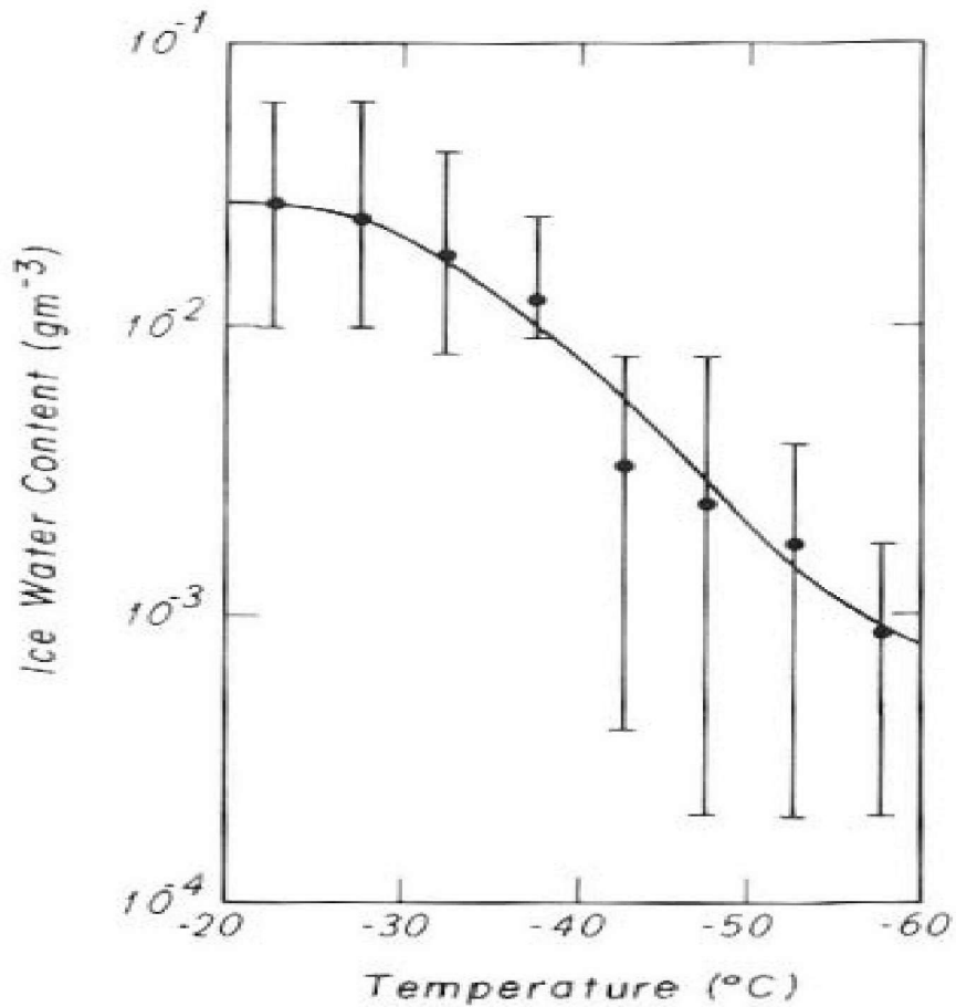
Figure 10. Mean ice water content for clouds found at temperatures between -20°C and -60°C (Liou 1992).
