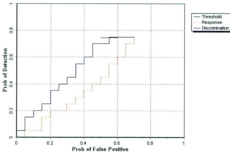
Figure 2. EM61 pushcart open field P_d^{\text{res}} and P_d^{\text{disc}} versus their respective BAR over all ordnance categories combined.
