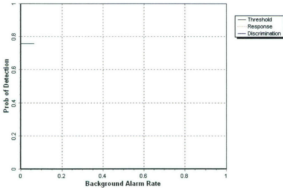
Figure 5. EM61 pushcart open field P_d^{\text{res}} and P_d^{\text{disc}} versus their respective \text{BAR}^{\text{res}} for all ordnance larger than 20 mm.
