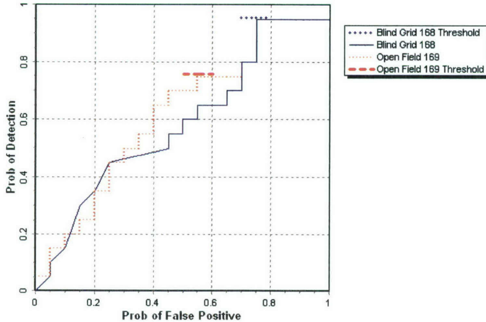
Figure 9. EM61 pushcart P_d^{\text{disc}} versus the respective P_{\text{fp}} for ordnance larger than 20 mm.
