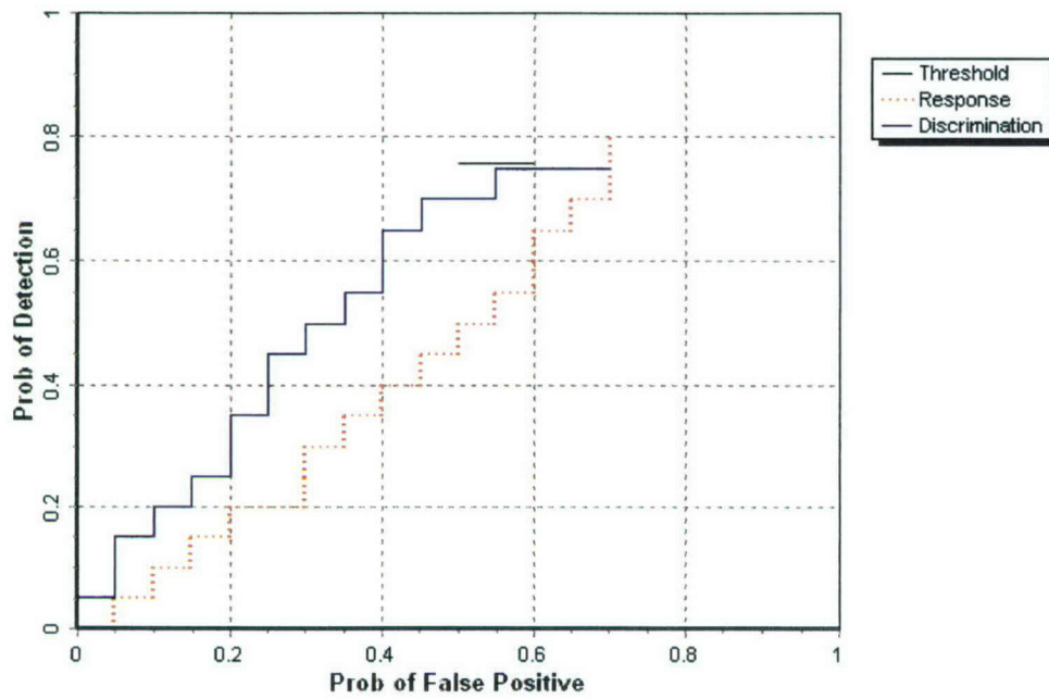
Figure 4. EM61 pushcart open field P_d^{\text{res}} and P_d^{\text{disc}} versus their respective P_{\text{fp}} for all ordnance larger than 20 mm.
