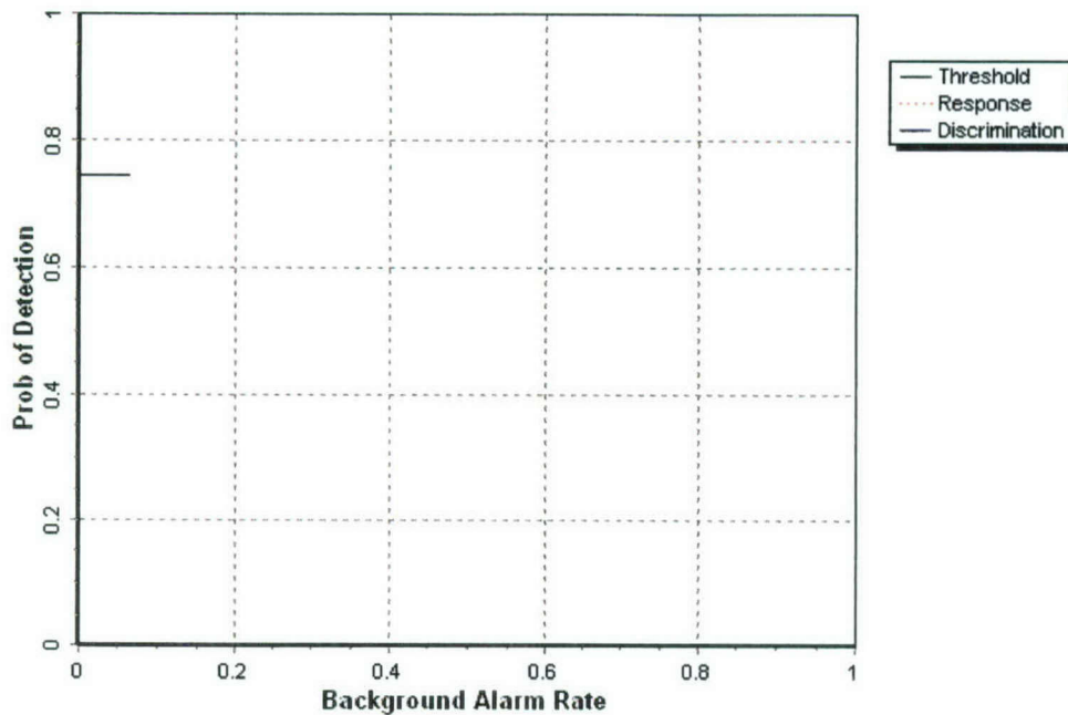
Figure 3. EM61 pushcart open field P_d^{\text{res}} and P_d^{\text{disc}} versus their respective BAR over all ordnance categories combined.
