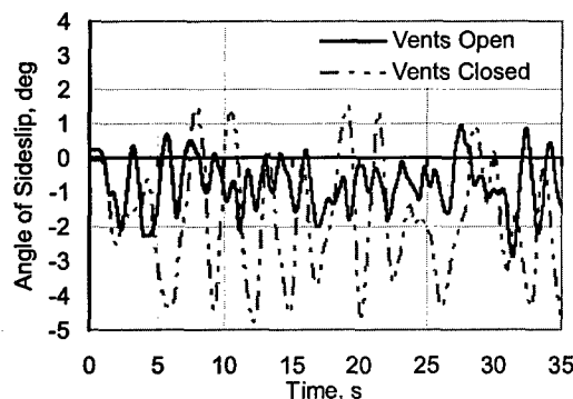
Figure 11. \beta time histories of the vents-opens and vents-closed configurations at \alpha = 16^\circ .
