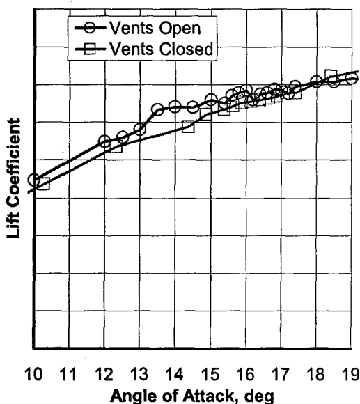
Figure 8. Lift characteristics for the vents-open and vents-closed configurations.
