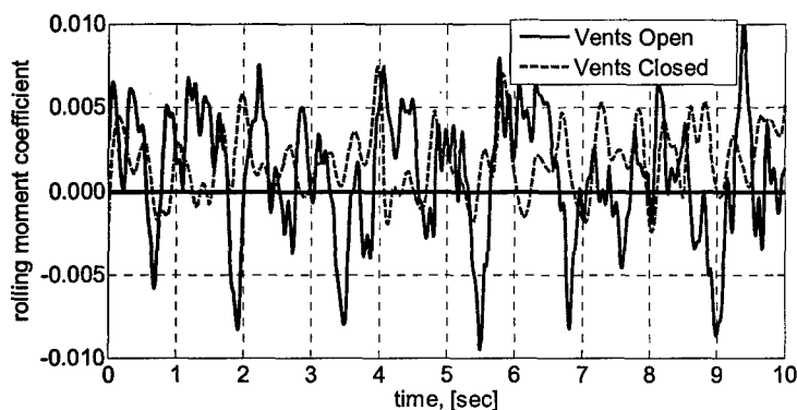
Figure 5. Balance rolling moment time history for vents open and vents closed, \alpha = 12^\circ .
