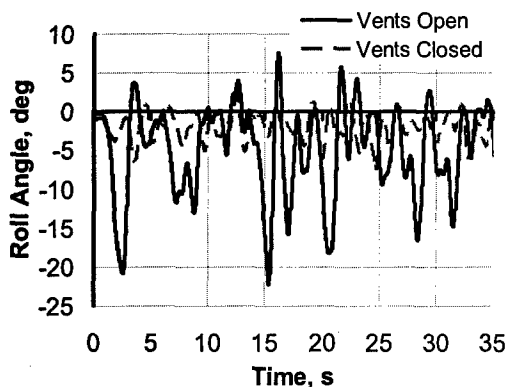
Figure 3. Roll angle time histories for the vents-open and -closed configurations at \alpha = 13^\circ .
