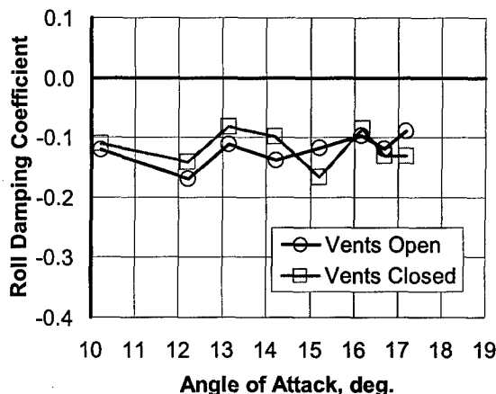
Figure 7. Effect of vents on roll damping.
