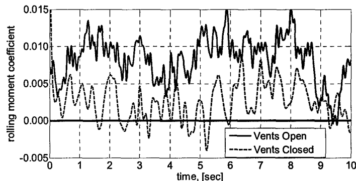
Figure 12. Balance rolling moment time history for vents open and vents closed, \alpha = 16^\circ .
