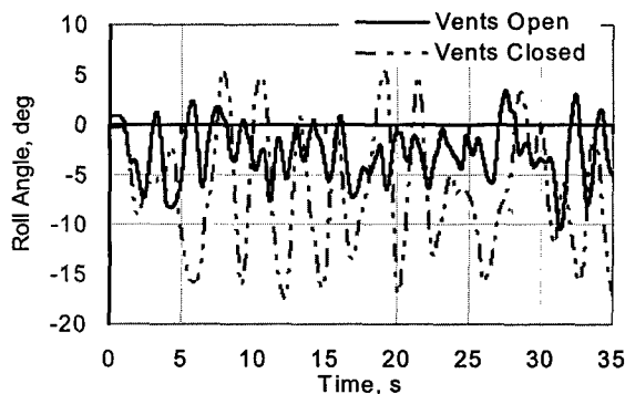
Figure 9. Roll angle time histories of the vents-open and vents-closed configurations at \alpha = 16^\circ .
