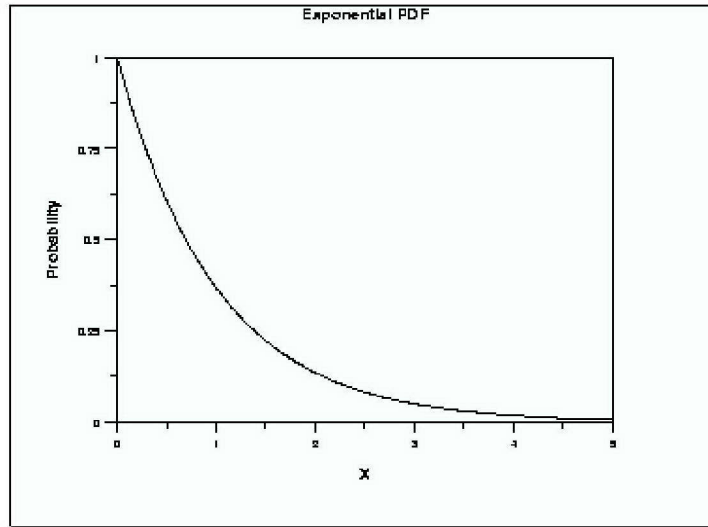
Figure 17. Exponential probability density (From Ref. [17].)
