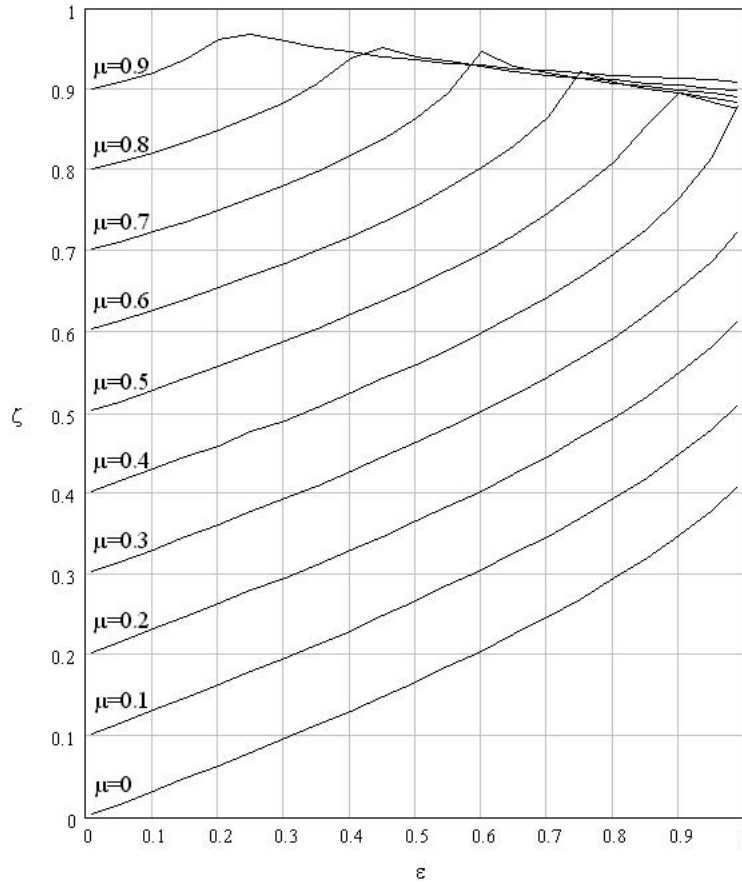
Figure 3.14 Variable Stiffness Constant Damping Optimal Equivalent Damping Ratio
