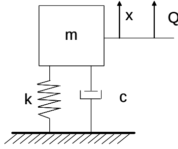
Figure 2.1 SDOF Suppression Problem with Constant Parameters
