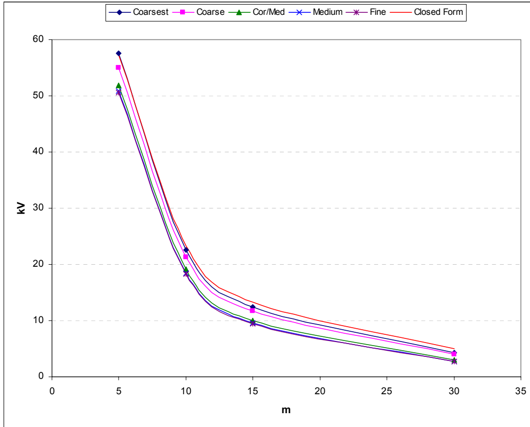
Figure 15. Effective volume ( k_V \cdot V ) as a function of the Weibull modulus and mesh.
