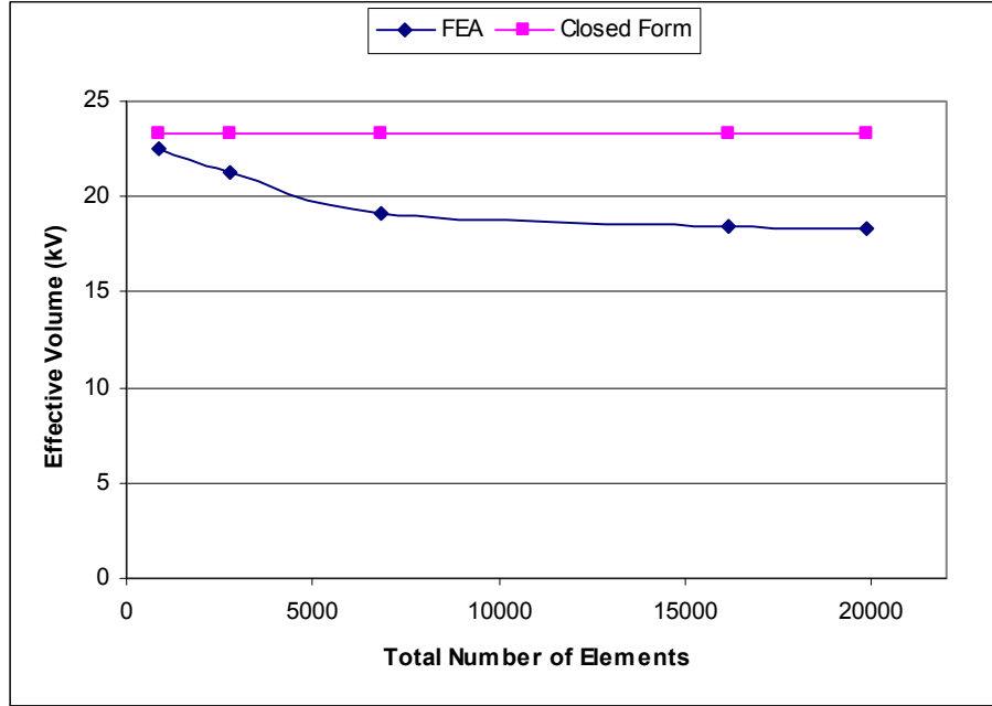
Figure 17. Effective volume as a function of mesh size for m = 10 .
