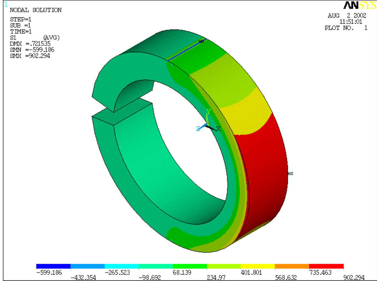
Figure 3. Principal stress contour map.
