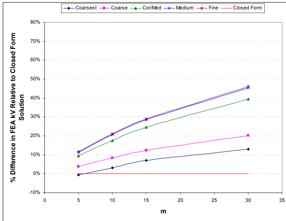
Figure 16. Percentage difference in ( k_V \cdot V ) as a function of mesh size and Weibull modulus.
