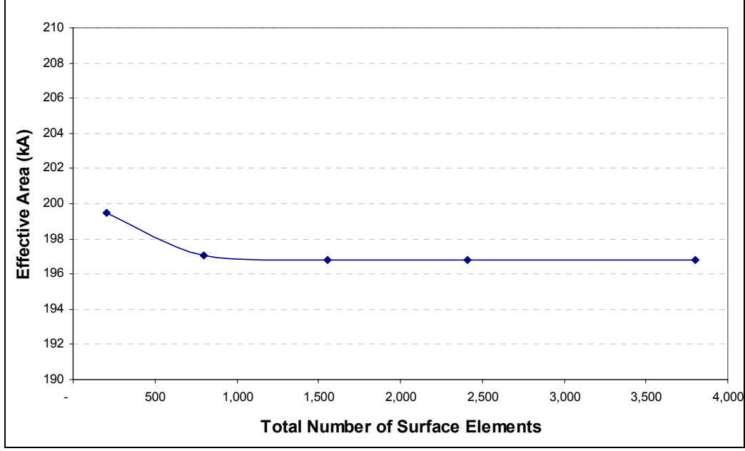
Figure 24. Effective area as a function of mesh density for m = 10 .
