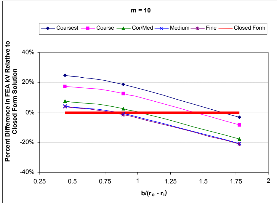
Figure 19. Percentage difference in effective volume relative to the closed form solution as a function of specimen geometry for m = 10 .
