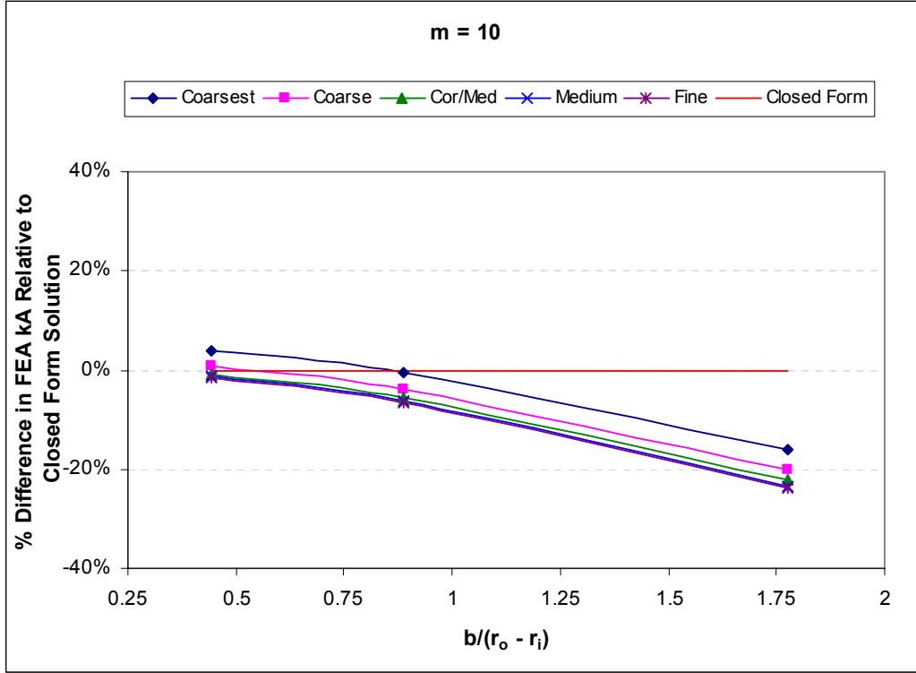
Figure 20. Percentage difference in effective area ( k_A \cdot A ) relative to the closed form solution as a function of specimen geometry for m = 10 .
