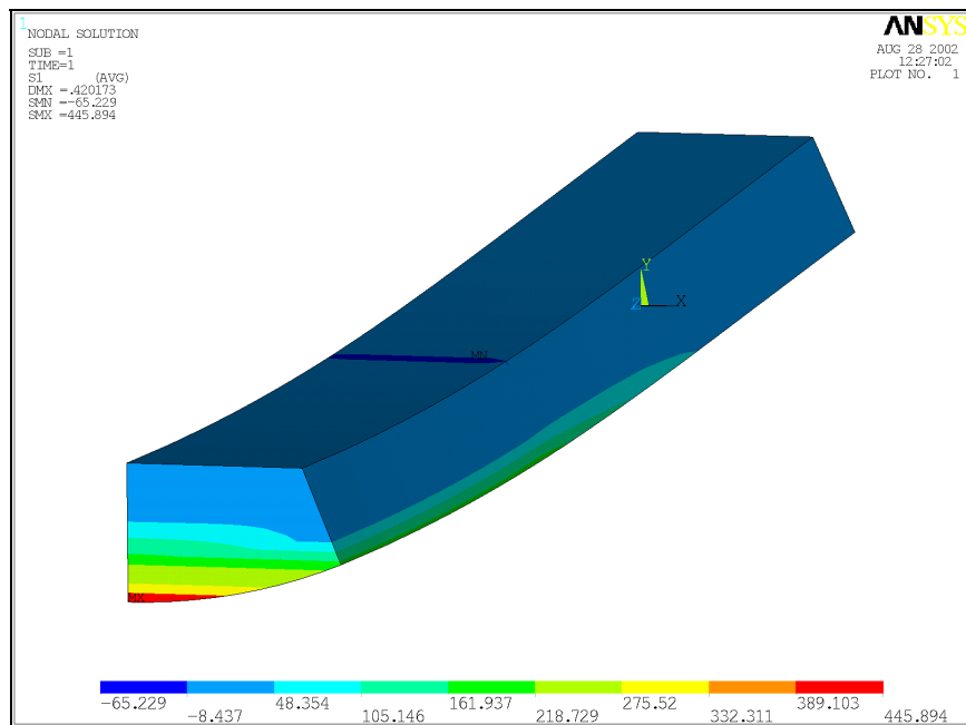
Figure 14. Principal stress contour plot.
