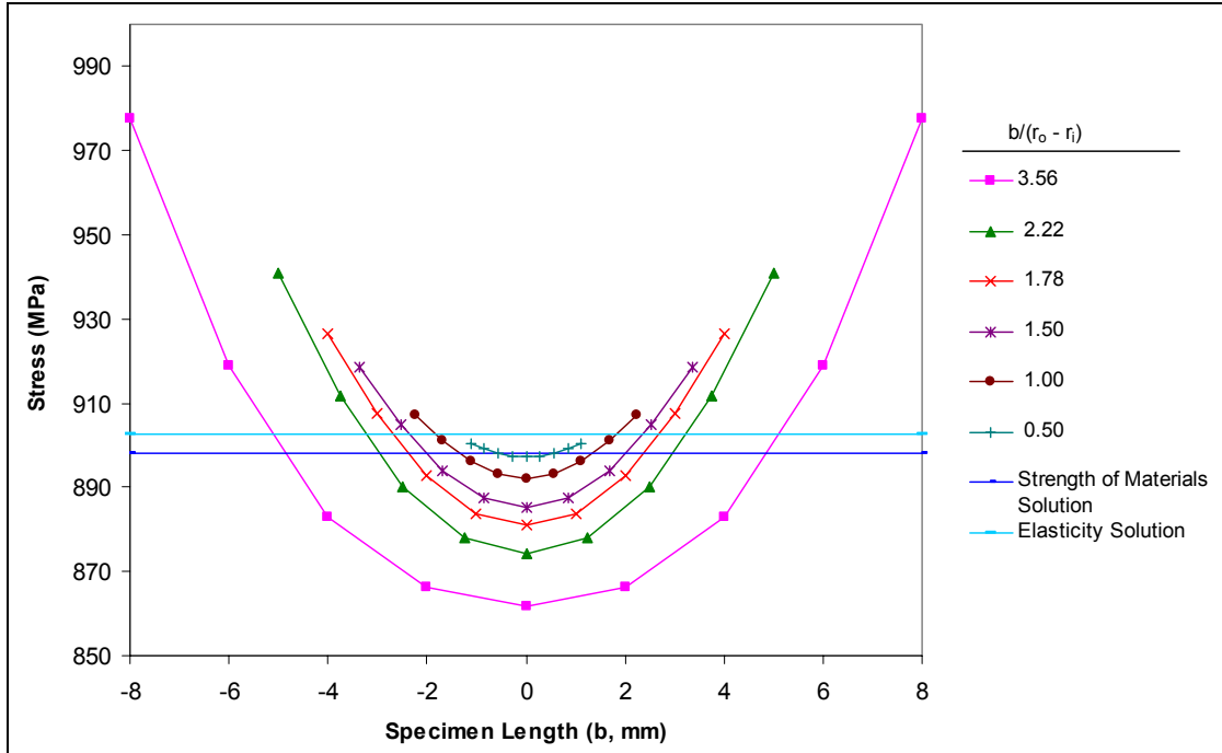
Figure 5. Maximum circumferential tensile stress as a function of specimen geometry.
