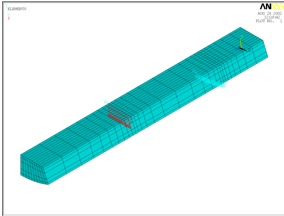
Figure 11. Most coarse quarter symmetry mesh with applied forces.
