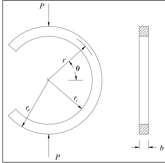
Figure 4. Schematic of C-ring specimen geometry.
