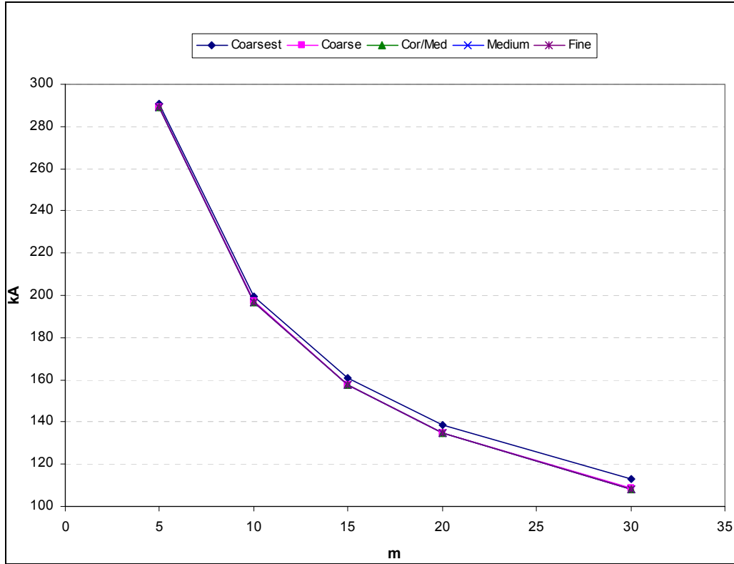
Figure 23. Effective area ( k_A \cdot A ) as a function of the Weibull modulus and mesh density.
