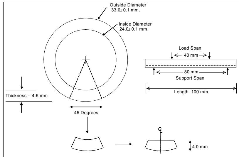
Figure 7. Sectoried tube geometry.
