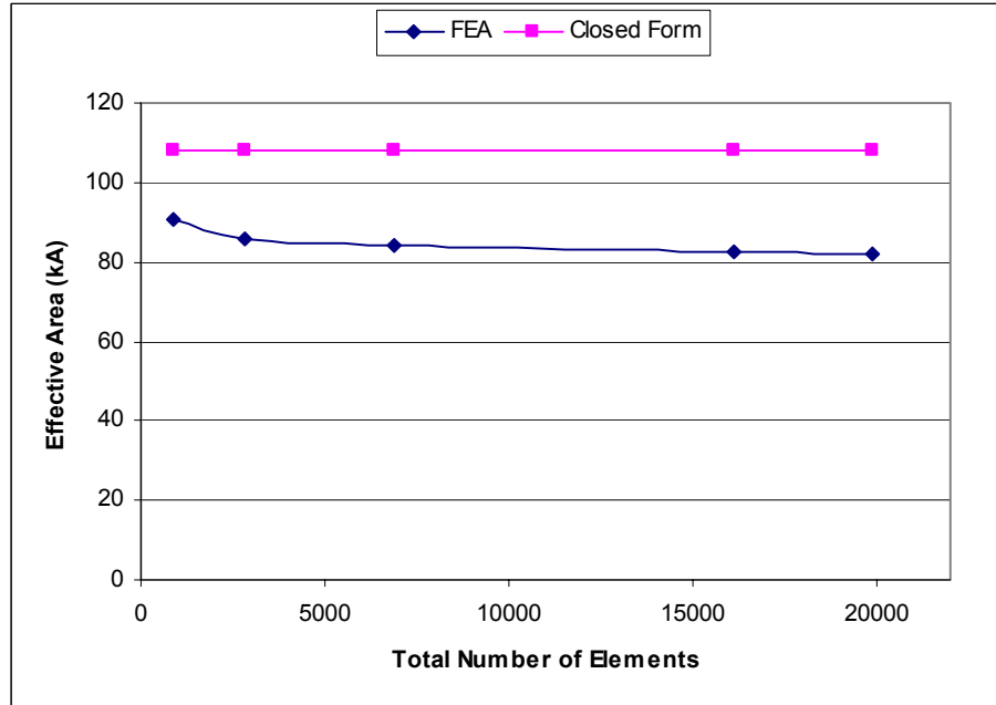
Figure 19. Effective area ( k_A \cdot A ) as a function of mesh size for m = 10 .
