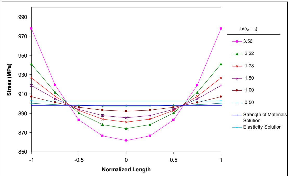
Figure 6. Maximum circumferential tensile stress as a function of specimen geometry normalized with respect to specimen length.
