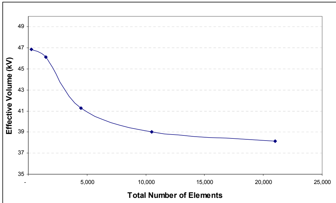
Figure 22. Effective volume as a function of mesh density for m = 10 .
