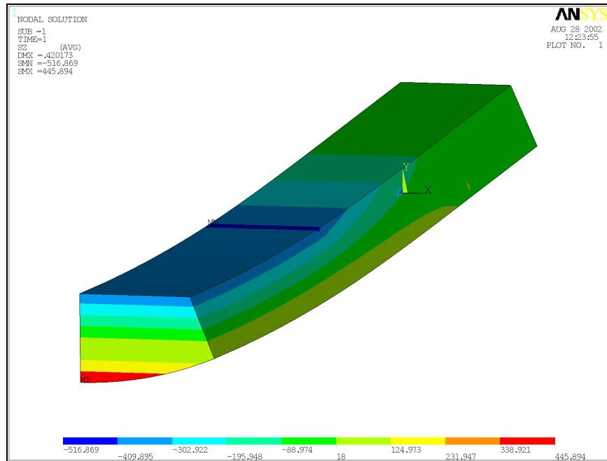
Figure 13. Z-axis stress contour plot.
