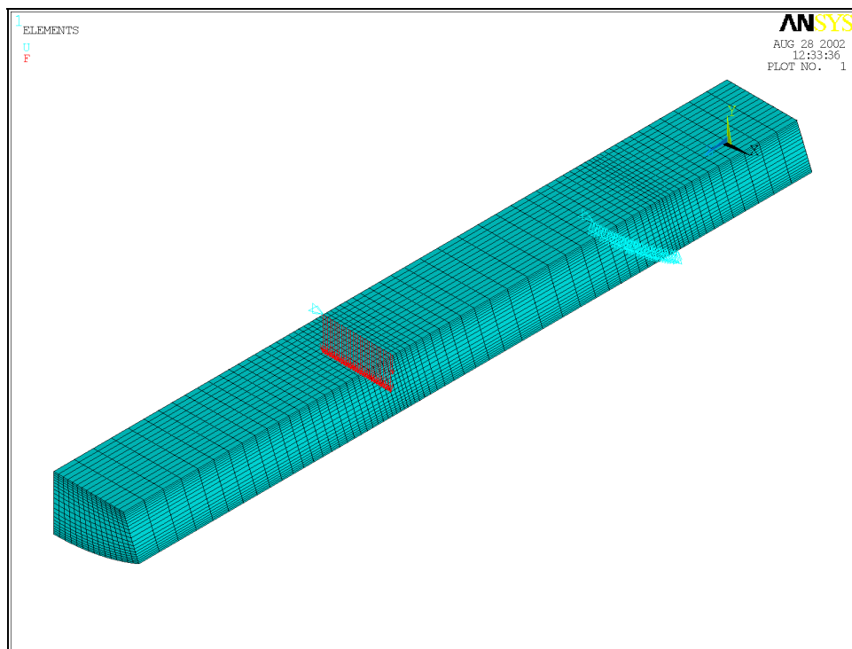
Figure 12. Most refined quarter symmetry mesh with applied forces.
