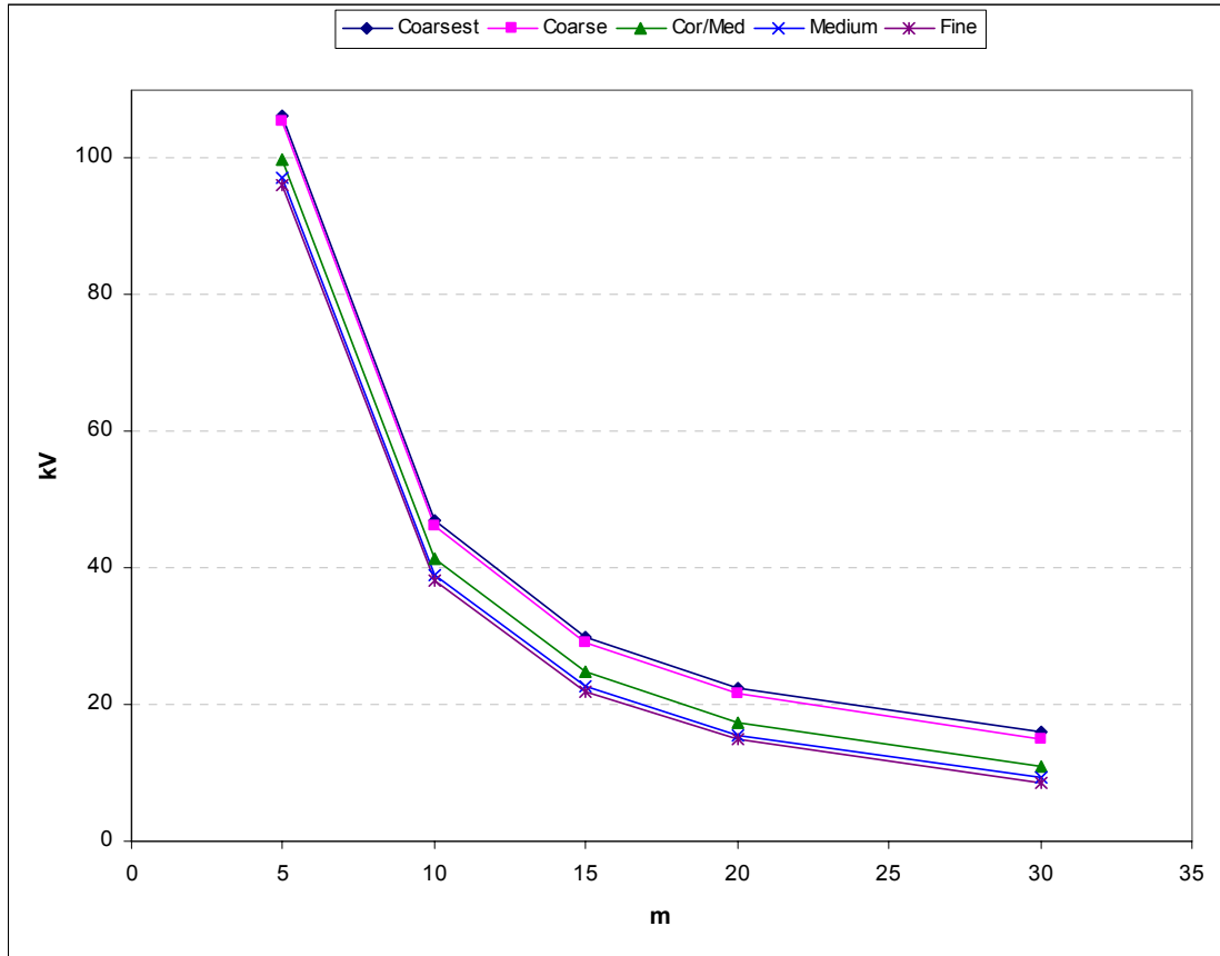
Figure 21. Effective volume ( k_V \cdot V ) as a function of the Weibull modulus and mesh density.
