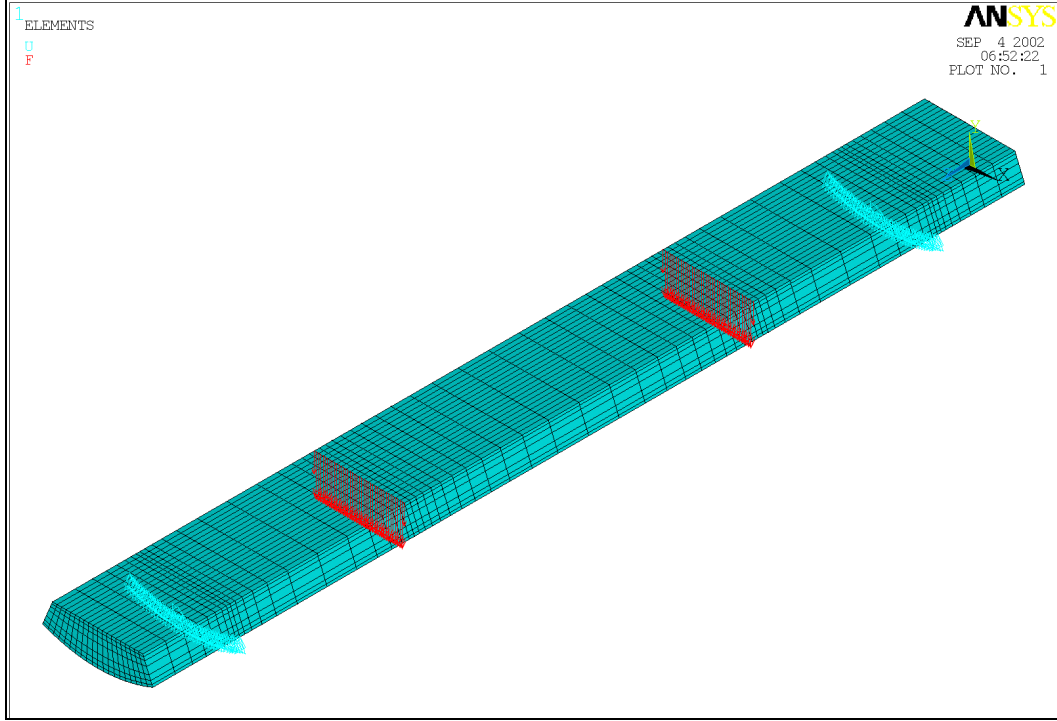
Figure 9. Full model with applied forces.
