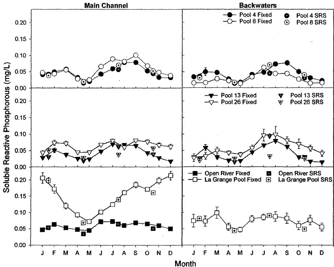
Figure 4.3. Monthly mean (1993–2001) soluble reactive phosphorous (mg/L) concentrations in the main channel and backwaters of the Upper Mississippi and Illinois Rivers. Monthly data are from fixed-site sampling. Stratified random sampling (SRS) points are plotted quarterly between the 2 months that the 2-week SRS episode spans. Error bars represent \pm one standard error.
