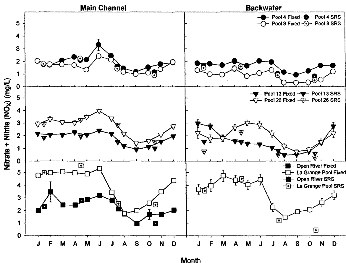
Figure 4.4. Monthly mean (1993–2001) nitrate + nitrite (mg/L; \text{NO}_x ) concentrations in the main channel and backwaters of the Upper Mississippi and Illinois Rivers. Monthly data are from fixed-site sampling. Stratified random sampling (SRS) points are plotted as in Figure 4.3. Error bars represent \pm one standard error.
