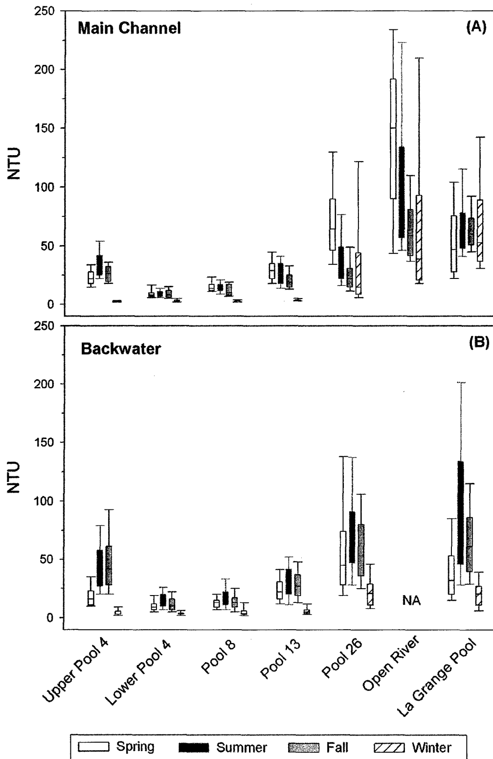
Figure 3.2. Box plots of winter, spring, summer, and fall turbidity (in nephelometric turbidity units [NTU]) in (A) main channel and (B) backwaters in the Long Term Resource Monitoring Program study reaches during stratified random sampling from 1993 through 2001. Box plots represent the 10th, 25th, 50th, 75th, and 90th percentiles.
