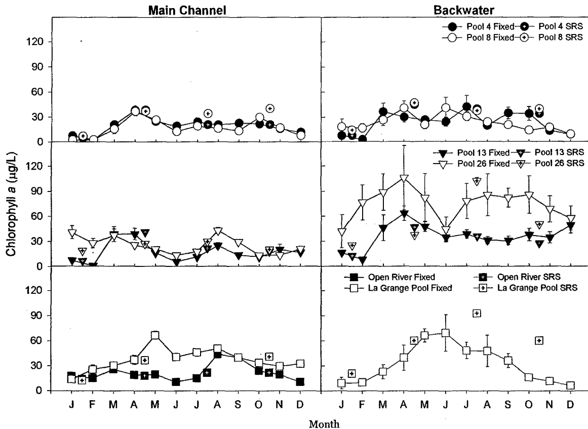
Figure 4.5. Monthly mean (1993–2001) chlorophyll a concentrations (µg/L) in the main channel and backwaters of the Upper Mississippi and Illinois Rivers. Monthly data are from fixed-site sampling. Stratified random sampling (SRS) points are plotted as in Figure 4.3. Error bars represent +/- one standard error.
