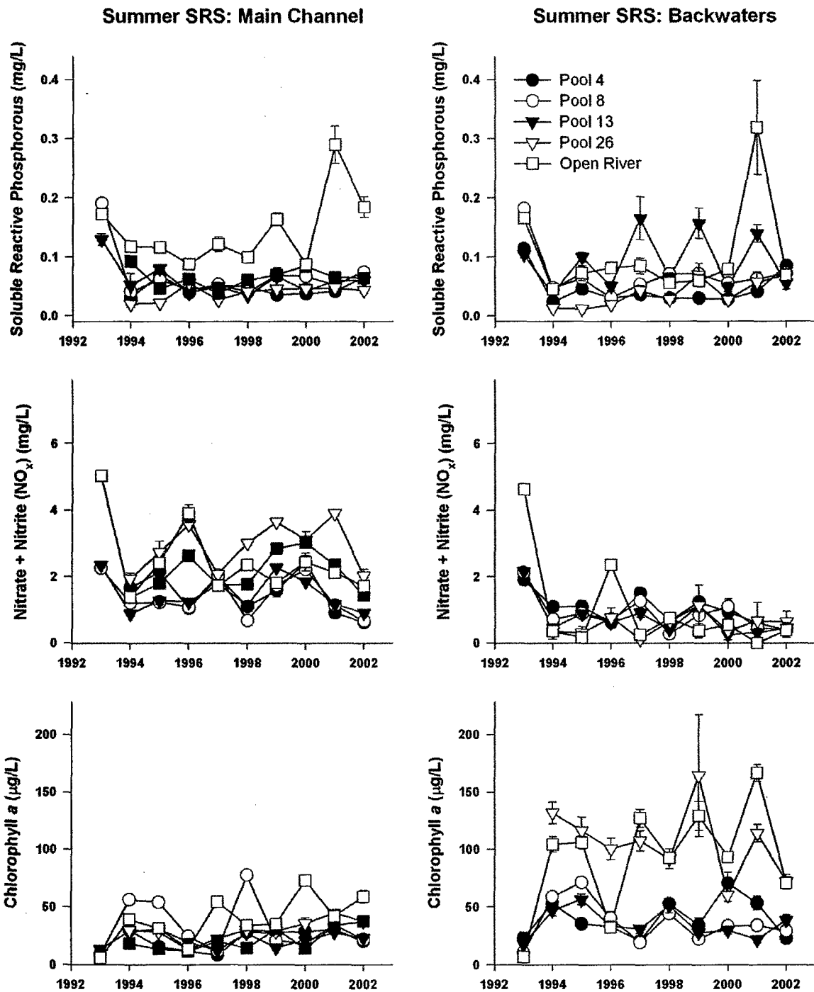
Figure 4.2. Annual means of soluble reactive phosphorous (mg/L), nitrate + nitrite nitrogen (mg/L; \text{NO}_x ), and chlorophyll a ( \mu\text{g/L} ) in the main channel and backwaters of the Upper Mississippi and Illinois Rivers based on summer stratified random sampling (SRS) from 1993 to 2002. Error bars represent +/- one standard error.
