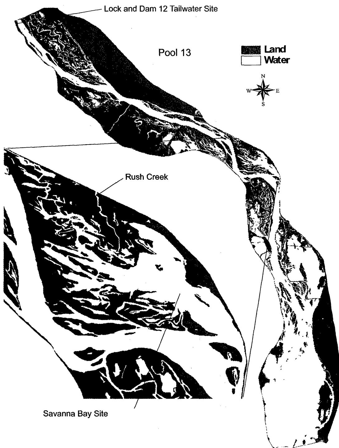
Figure 6.5. Pool 13 of the Upper Mississippi River showing the Lock and Dam 12 tailwater site, Savanna Bay site, and Rush Creek. Inset map shows spatial relation of Rush Creek to the Savanna Bay site.
