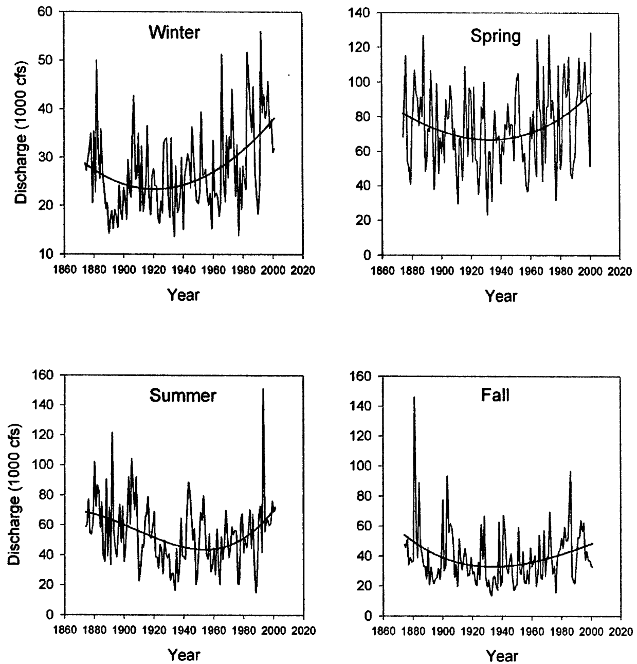
Figure 2.4. Yearly seasonal mean discharge (cfs) at Clinton, Iowa, for a 128-year period (1874–2001). The fitted line represents a third-order polynomial relation.
