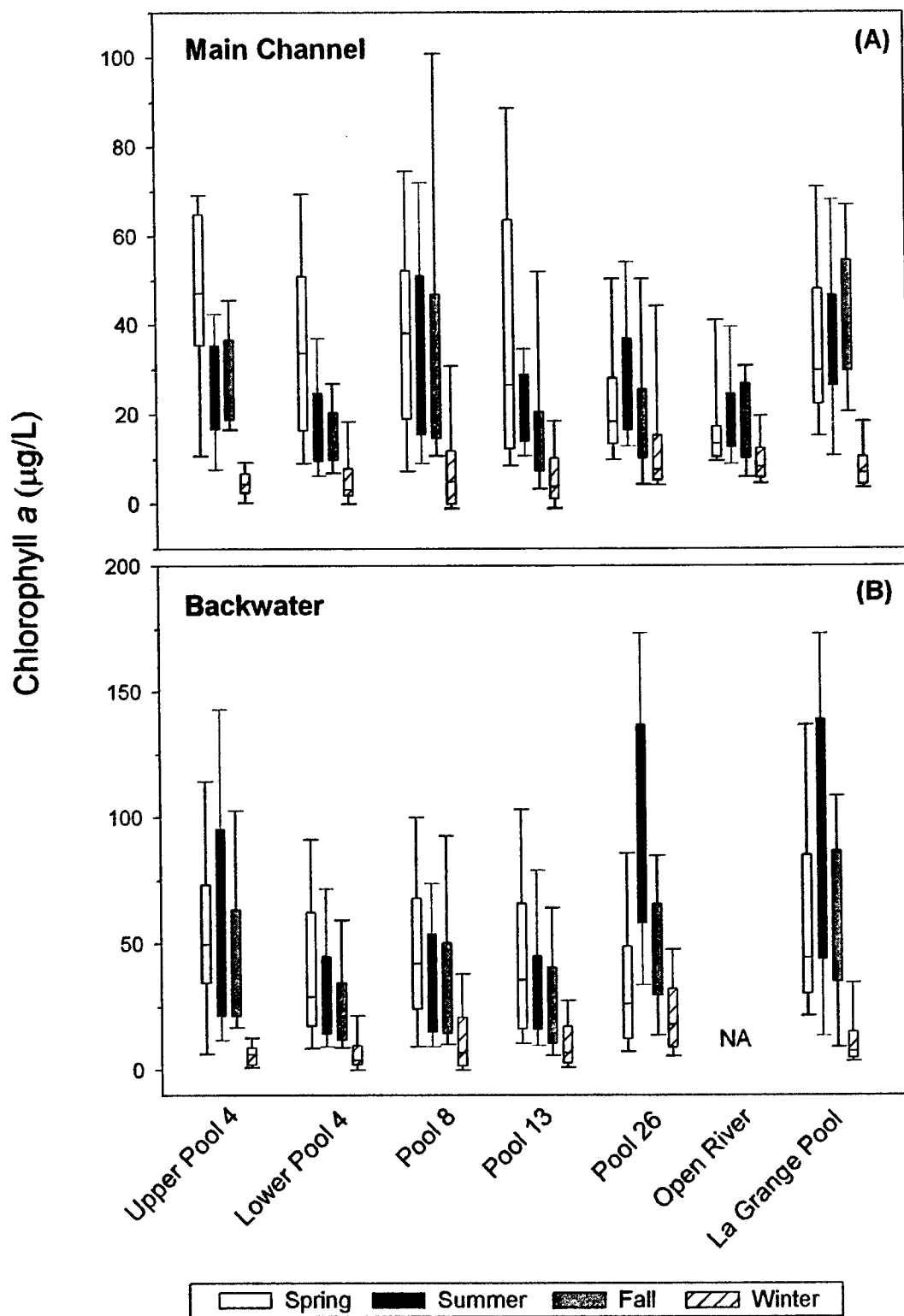
Figure 3.3. Box plots of winter, spring, summer and fall chlorophyll a concentrations (µg/L) in (A) main channel and (B) backwaters in the Long Term Resource Monitoring Program study reaches during stratified random sampling from 1993 through 2001. Box plots represent the 10th, 25th, 50th, 75th, and 90th percentiles.
