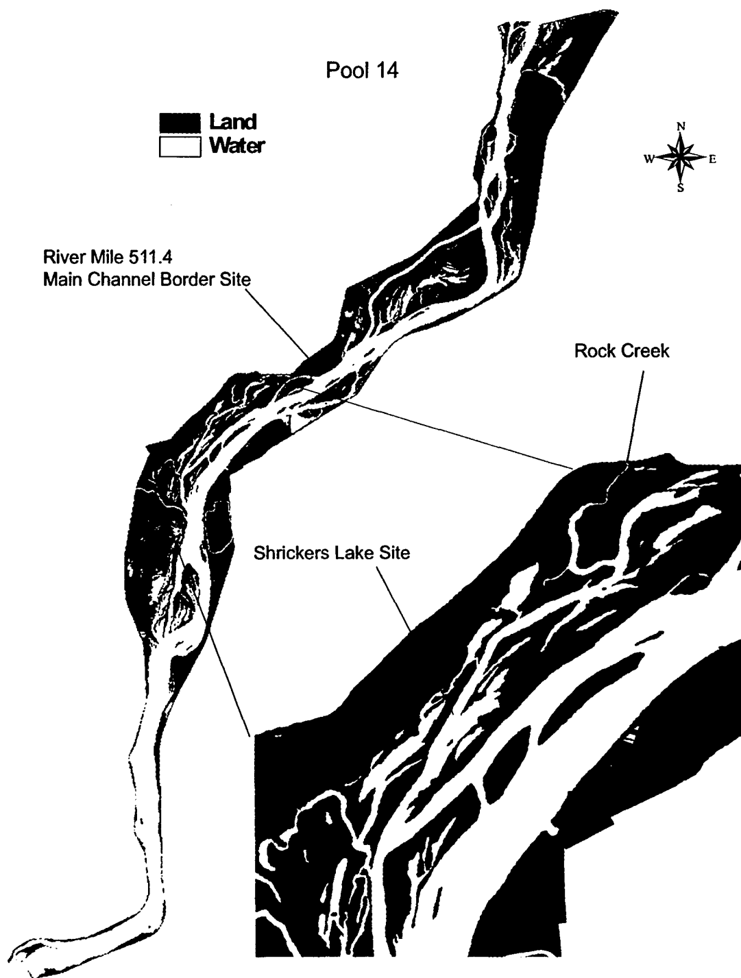
Figure 6.6. Pool 14 of the Upper Mississippi River showing Pool 14 main channel border fixed-site sampling, Shrickers Lake site, and Rock Creek. Inset map shows spatial relation of Rock Creek to the Shrickers Lake site.
