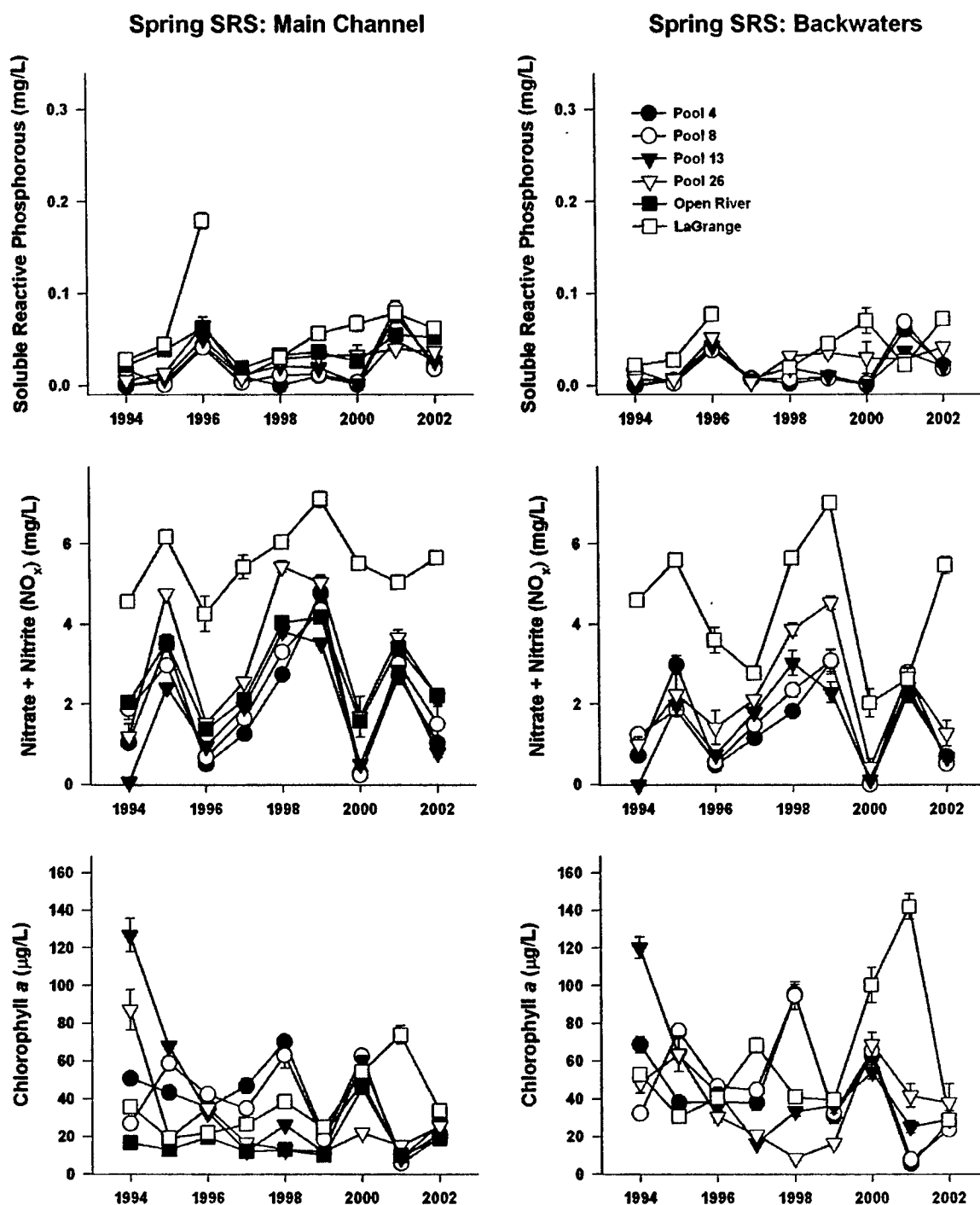
Figure 4.1. Annual means of soluble reactive phosphorous (mg/L), nitrate + nitrite oxygen (mg/L; \text{NO}_x ), and chlorophyll a ( \mu\text{g/L} ) in the main channel and backwaters of the Upper Mississippi and Illinois Rivers based on spring stratified random sampling (SRS) from 1994 to 2002. Error bars represent \pm one standard error.
