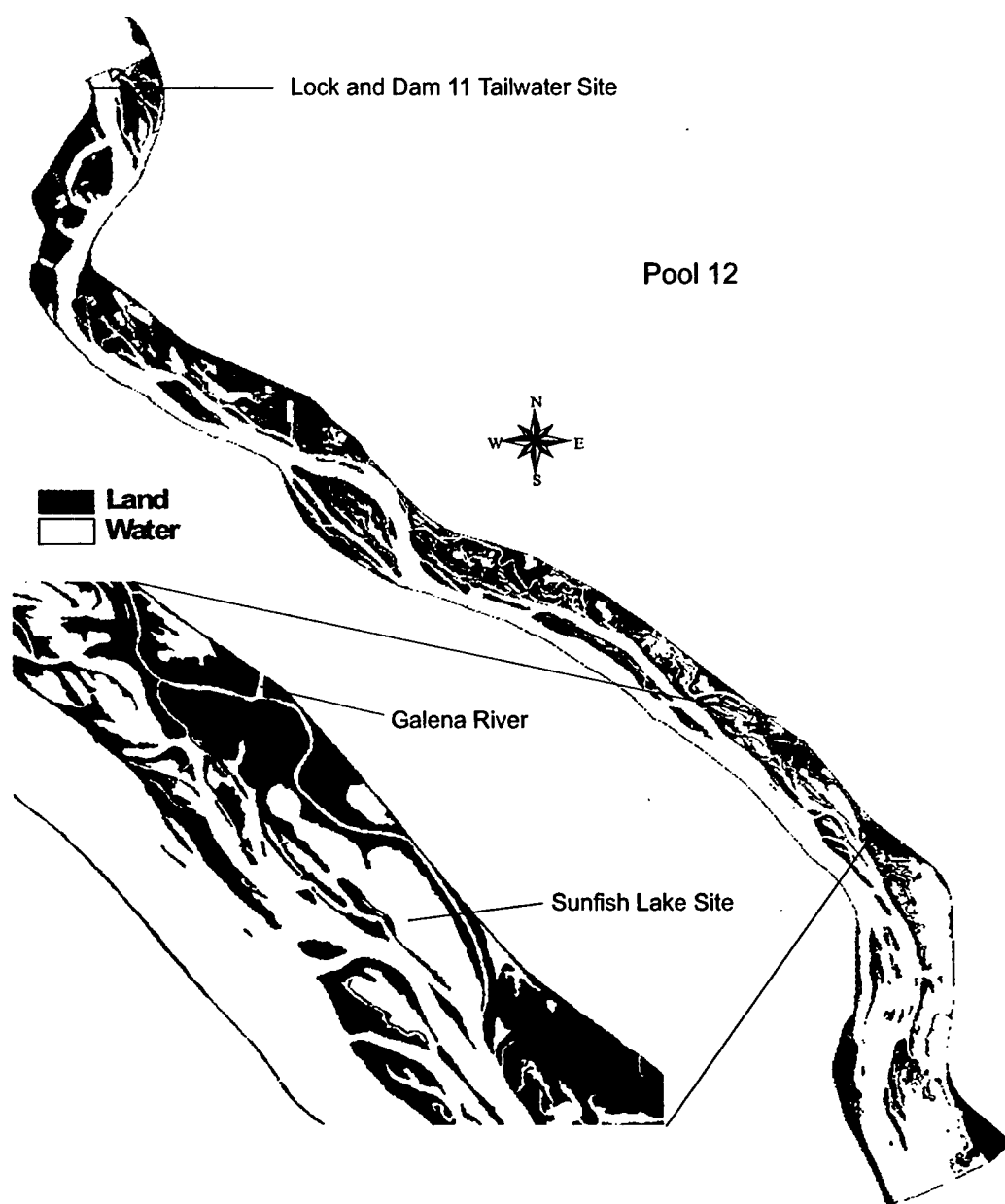
Figure 6.4. Pool 12 of the Upper Mississippi River showing the Lock and Dam 11 tailwater site, Sunfish Lake site, and the Galena River. Inset map shows spatial relation of the Galena River to the Sunfish Lake site.
