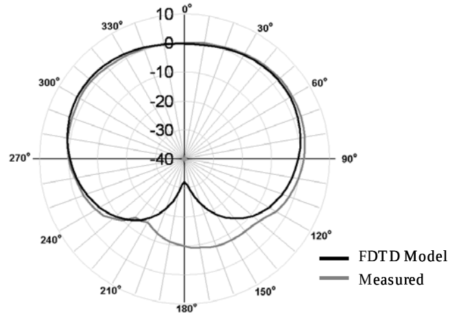
Fig5. Iridium validated antenna model pattern results.
