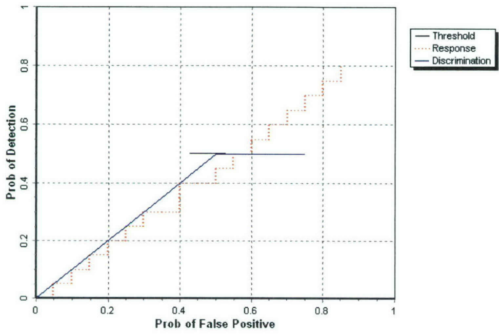
Figure 4. TM-5 EMU Open Field P_d^{res} and P_d^{disc} versus their respective P_{fp} for all ordnance larger than 20 mm.
