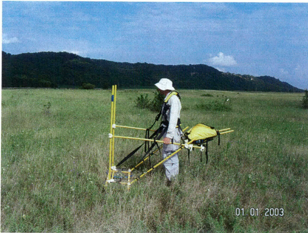
Figure 1. Demonstrator's system, TM-5 EMU (dual-sensor).
