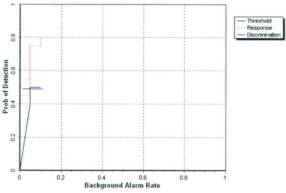
Figure 5. TM-5 EMU Open Field P_d^{res} and P_d^{disc} versus their respective BAR^{res} for all ordnance larger than 20 mm.
