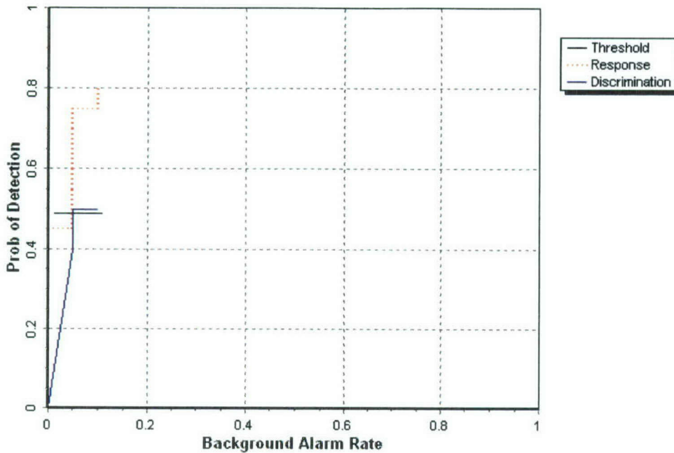
Figure 3. TM-5 EMU Open Field P_d^{\text{res}} and P_d^{\text{disc}} versus their respective BAR over all ordnance categories combined.
