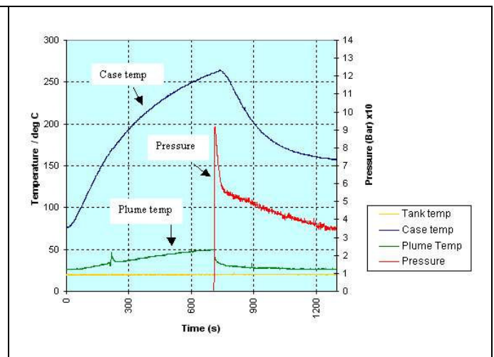
Figure 2.6: Butane flow data for AISAT-1 fight thruster, 15W input power
