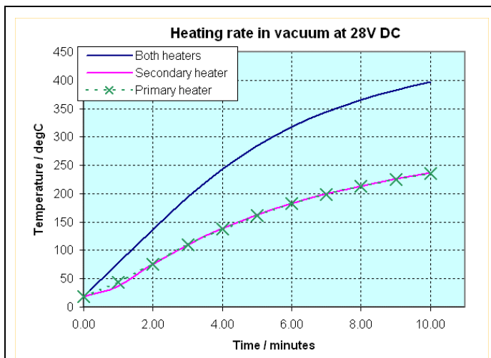
Figure 2.5: Heating rate measured on the AISAT flight thruster, 15 and 30W input power
