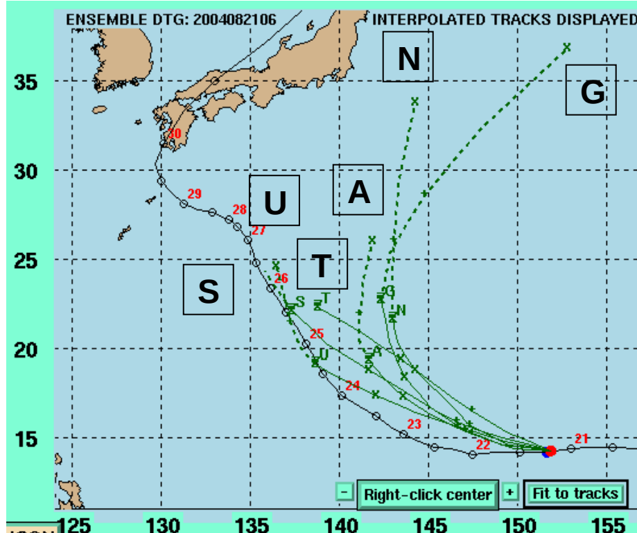
Figure 6. Interpolated forecast tracks for 19W by NOGAPS (N), GFDN (G), UKMO (U), the Global Spectral Model (S) and Typhoon Model (T) of the Japan Meteorological Agency, and GFS (A) for the forecast period of 0600 UTC 21 August 2004. The solid sections of the forecast tracks represent the 00-h through 72-h forecast while the dashed section represents the 72-h through 120-h forecast. The solid line with circles and corresponding dates represents the TC best track.
