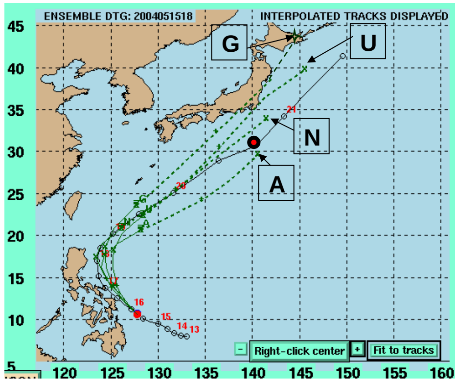
Figure 27. Interpolated forecast tracks for 04W by NOGAPS (N), GFDL (G), UKMO (U), and GFS (A) for the forecast of 1800 UTC 15 May 2004. The solid sections of the forecast tracks represent the 00-h through 72-h forecast while the dashed sections represent the 72-h through 120-h forecast. The solid line with open circles and corresponding dates represents the TC best track. The verifying 120-h position is indicated by the red circle with the heavy black outline.
