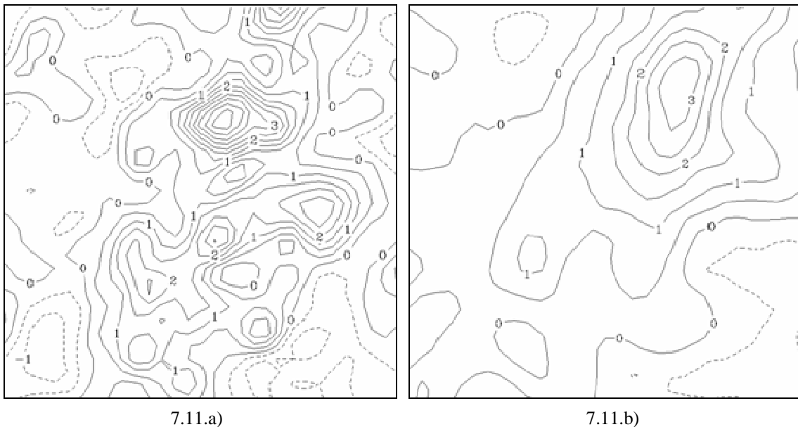
Figure 7.11. 21 hour divergence composites from MM5 and ETA-212 data, June-September 2004. 7.11.a) is the MM5 composite, and 7.11.b) is the ETA-212. Each image consists of a 375 km X 375 km area with a 0.5 contour interval.
