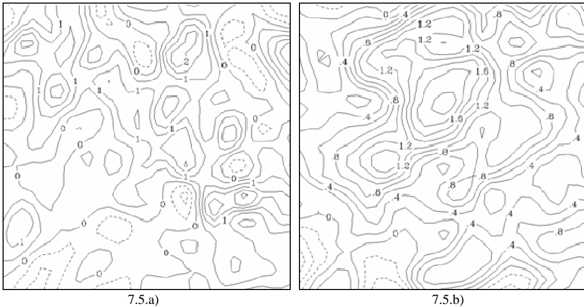
Figure 7.5. 12 hour divergence composites from MM5 and ETA-212 data, June-September 2004. 7.5.a) is the MM5 composite (0.5 contour interval), and 7.5.b) is the ETA-212 (0.2 contour interval).
