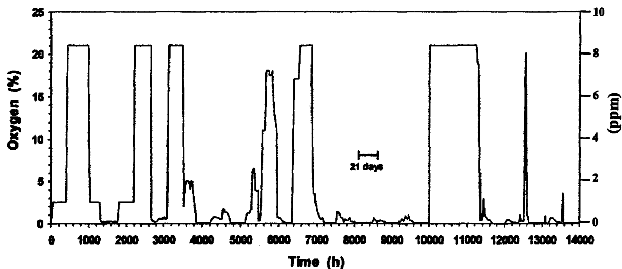
Figure 24. Dissolved oxygen concentration data from Matsuda's shipboard experiments of corrosion control using nitrogen to purge ballast tank headspace.
