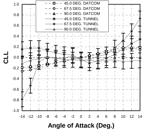
Figure 3: Rolling moment comparison
