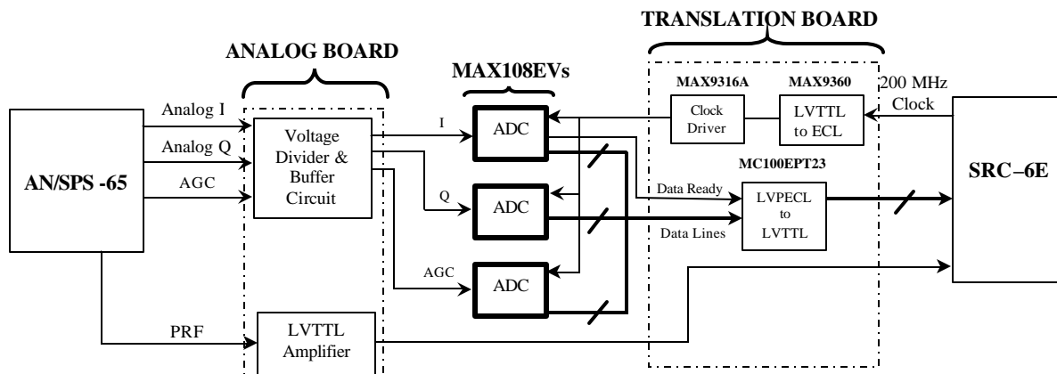
Figure 1. AN/SPS-65 to SRC-6E Hardware Interface Block Diagram
