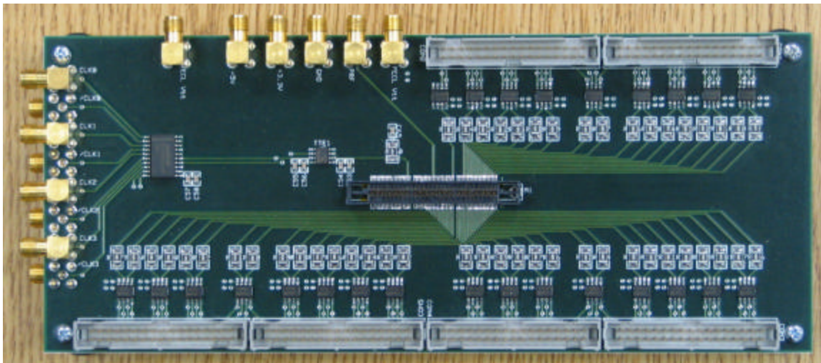
Figure 30. Assembled Translation Board
