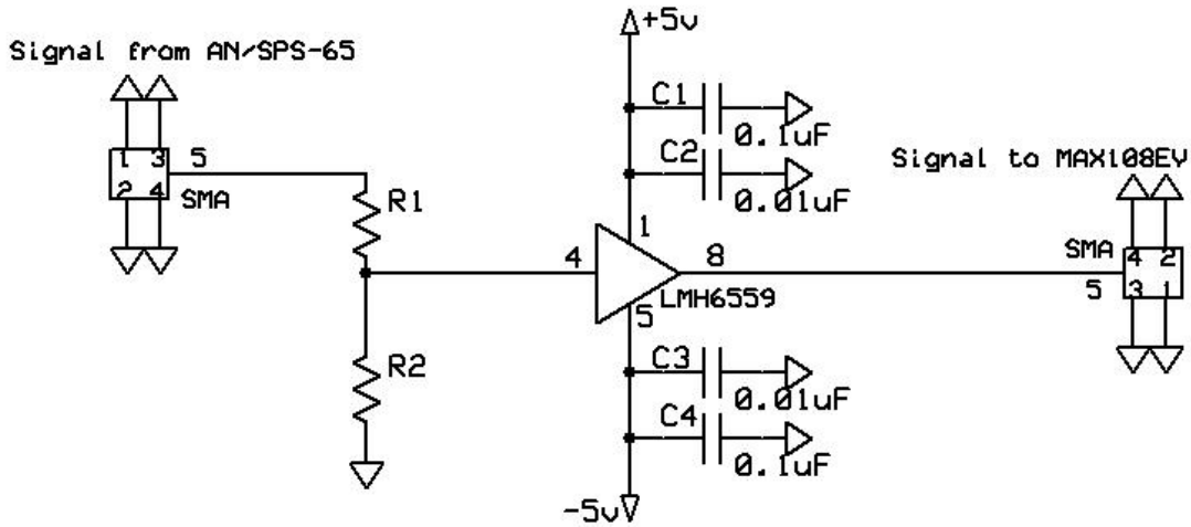
Figure 14. Two-Resistor Voltage Divider and Buffer Circuit
