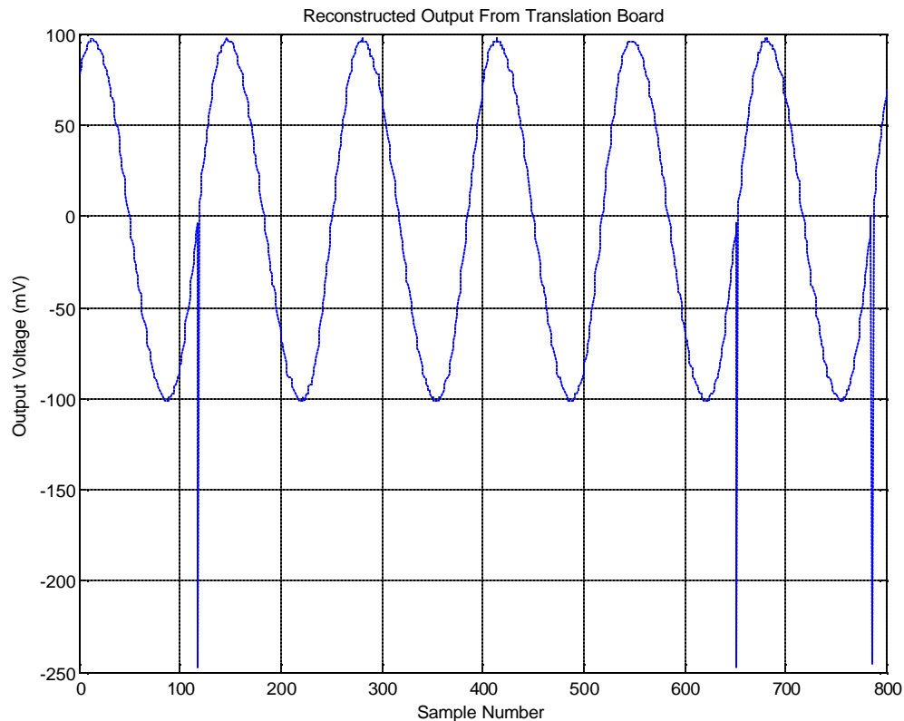
Figure 33. Translation Board Output with a 200-MHz Sample Clock
