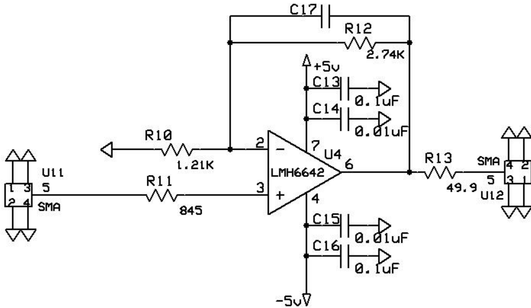
Figure 16. PRF Timing Reference LVTTL Amplification Circuit
