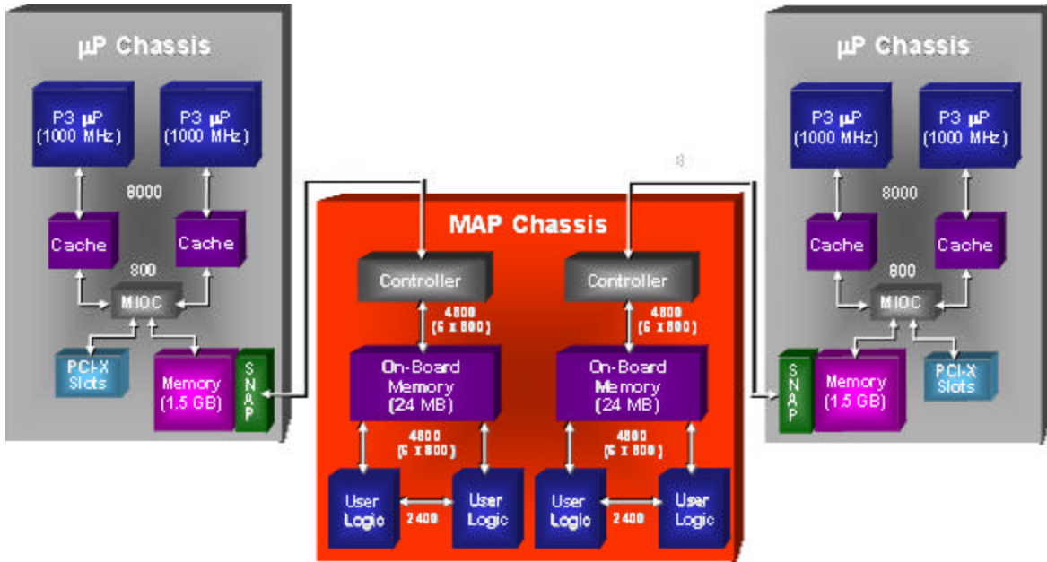
Figure 2. SRC-6E System Architecture Block Diagram (From Ref. 5.)
