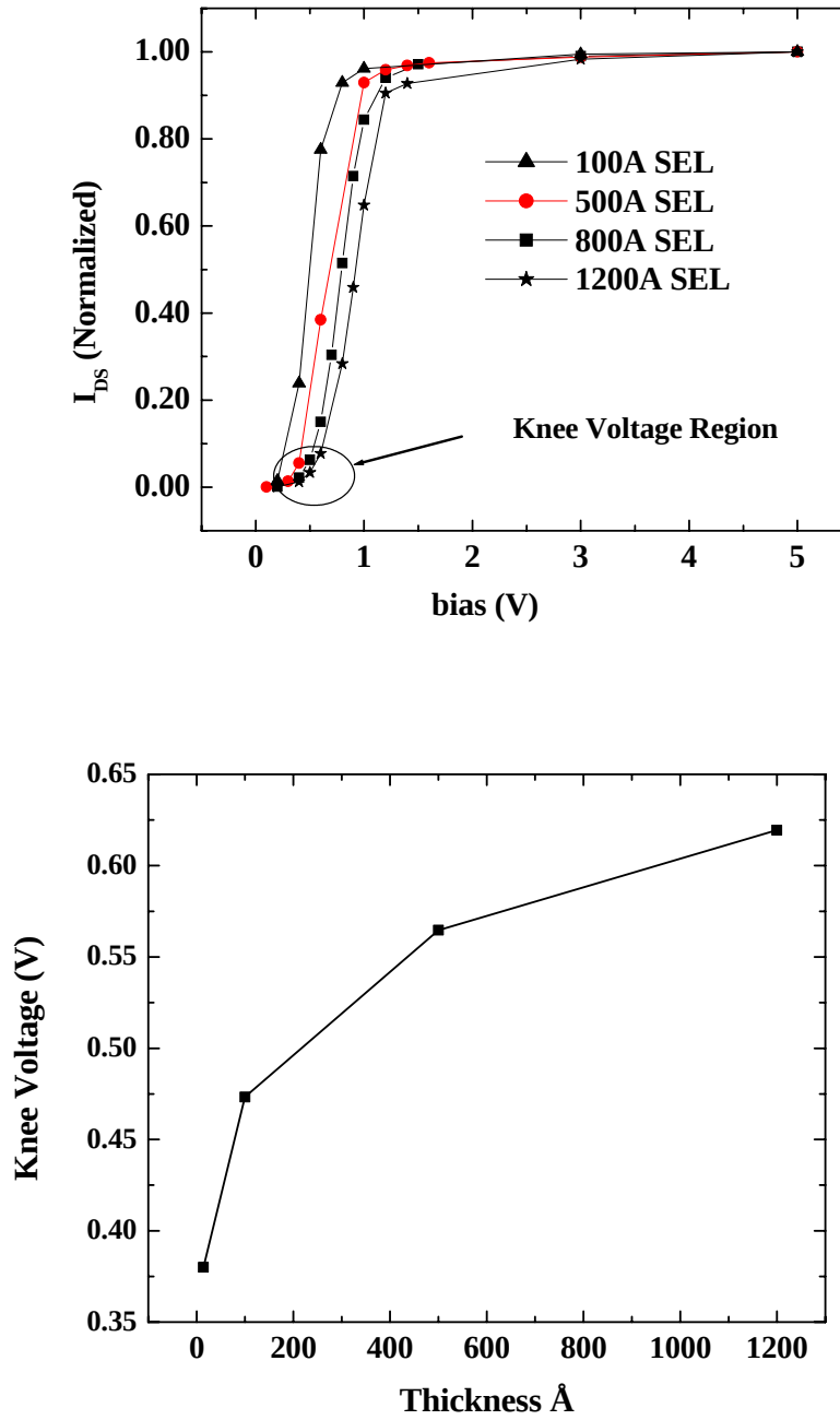
Figure 23. (top) Simulated DC responsivity of a 60\text{ }\mu\text{m} \times 60\text{ }\mu\text{m} MSM photodetector with 3\text{ }\mu\text{m} finger width and 3\text{ }\mu\text{m} finger spacing for different SEL thicknesses at 14\text{ }\mu\text{W} of the light intensity. (bottom) Knee Voltage as a function of InAlAs layer SEL thickness.
