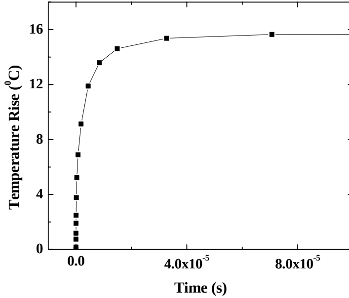
Figure 9. Transient characteristics of the VCSEL when the current is switched on from 0 to 10 mA.
