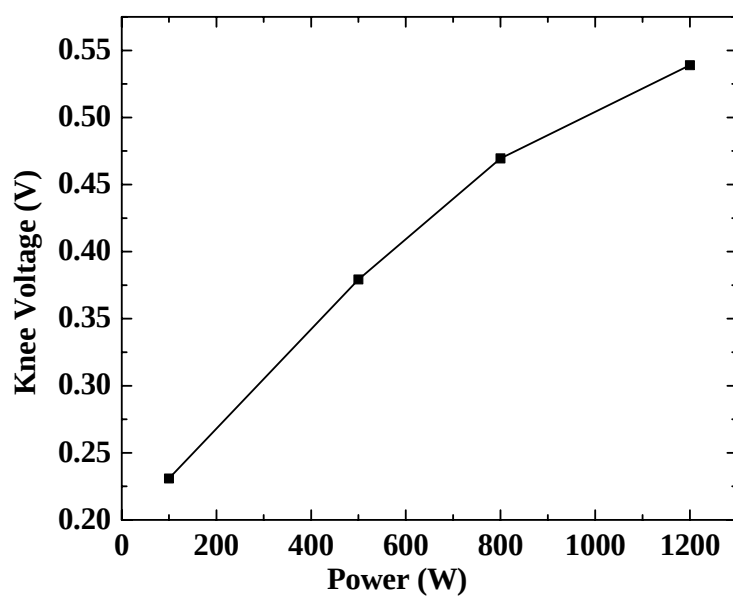
Figure 24. (top) Simulated DC response of InAlAs/InGaAs OE mixer for different light intensities. (bottom) Knee voltage as a function of power for 100 Å of InAlAs SEL.
