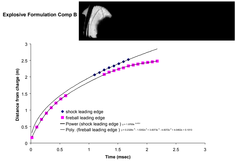
Figure 9: HBI imaging data from measurements of explosive formulation Comp B, showing shock and fireball leading edges as a function of time after initiation. Also shown in inset is an image of the leading shock and following fireball edge passing through the laser-illuminated region. Shock data (diamonds) and fireball leading edge data (rectangles) have best fit trend lines drawn through each point as an aid to the eye. Note separation distance between shock and fireball edges versus time.
