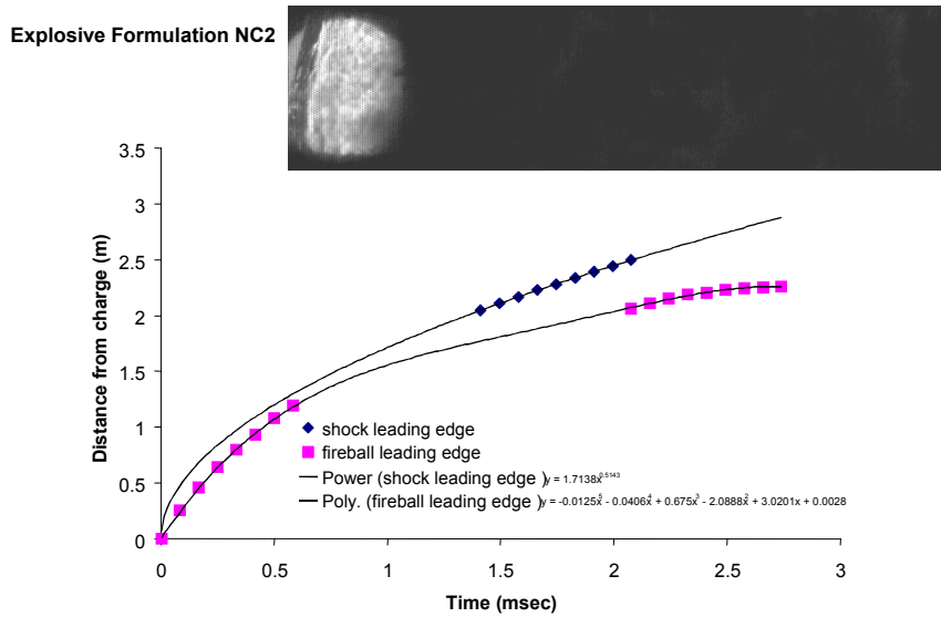
Figure 7: HBI imaging data from measurements of explosive formulation NC2, showing shock and fireball leading edges as a function of time after initiation. Also shown in inset is an image of the leading shock and following fireball edge passing through the laser-illuminated region. Shock data (diamonds) and fireball leading edge data (rectangles) have best fit trend lines drawn through each point as an aid to the eye. Note separation distance between shock and fireball edges versus time.
