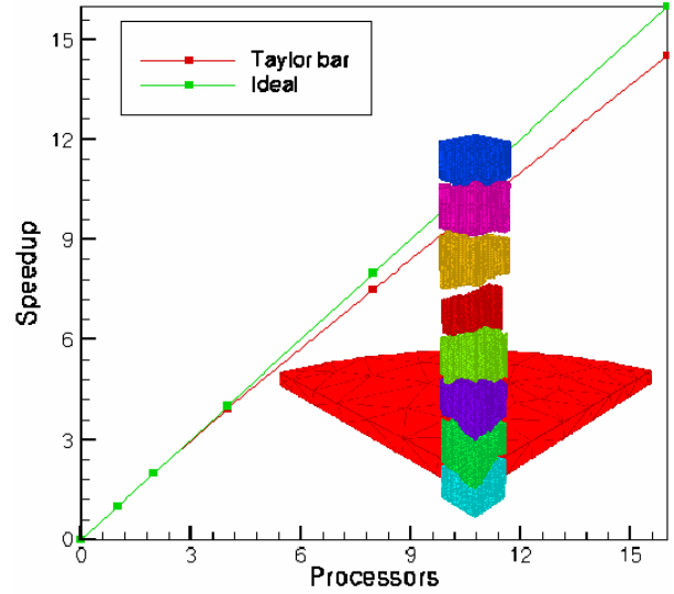
Figure 3: Initial parallel performance results for contact-impact problem - Taylor bar impact problem.
