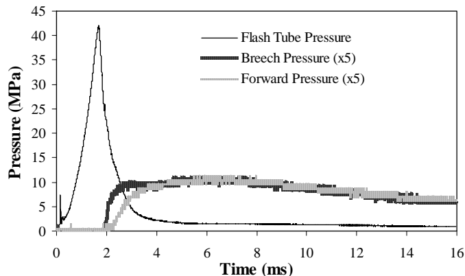
Fig. 5. Pressure-time histories for a properly functioning seal in the ballistic simulator
