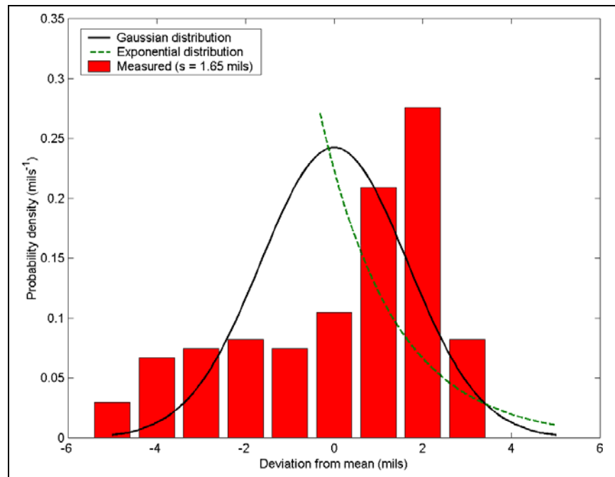
Figure 17. Measured surface height distribution of RHA plate 2-3, side A after coarse grit blasting compared to Gaussian and exponential distributions.
