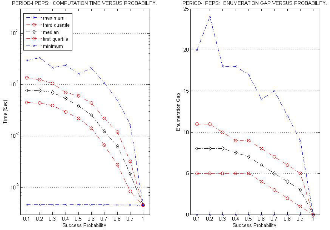
Figure 6. Period-I PEP Enumeration Versus Success Probability. The statistics presented are the same as in Figure 3. In each case, we set n=12 and |S^I|=12 . The probability threshold varies between 0.1 and 1. At lower success probabilities, the enumeration gap tends to be larger, resulting in longer computation times.
