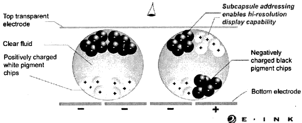
Figure 4. Cross-section diagram of E-Ink based display. (Source: E-Ink Corporation)
