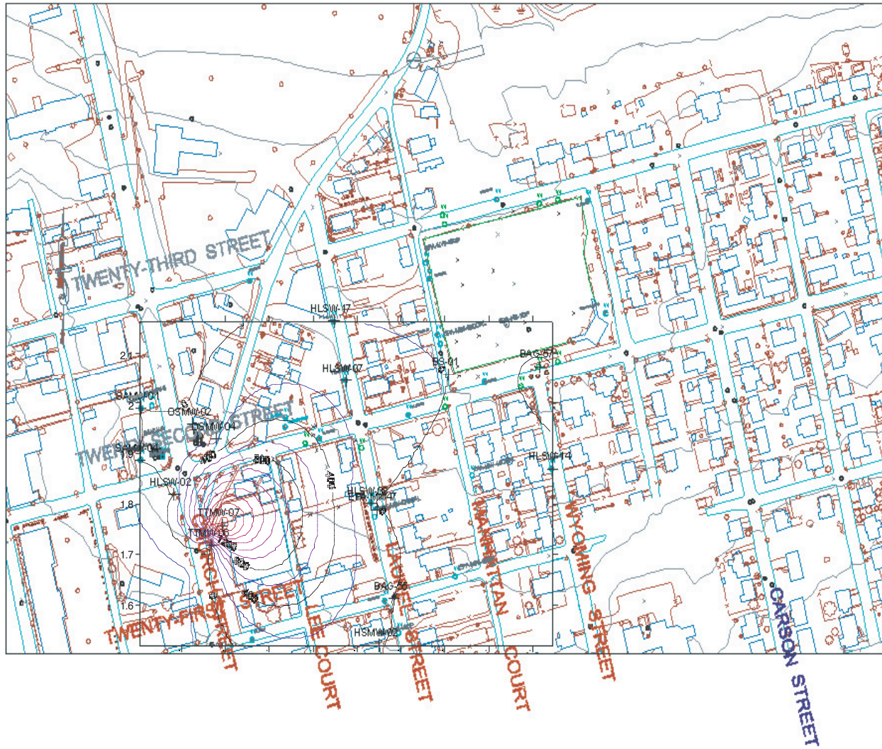
Fig. 9 — Benzene concentrations interpolated over sampling area
