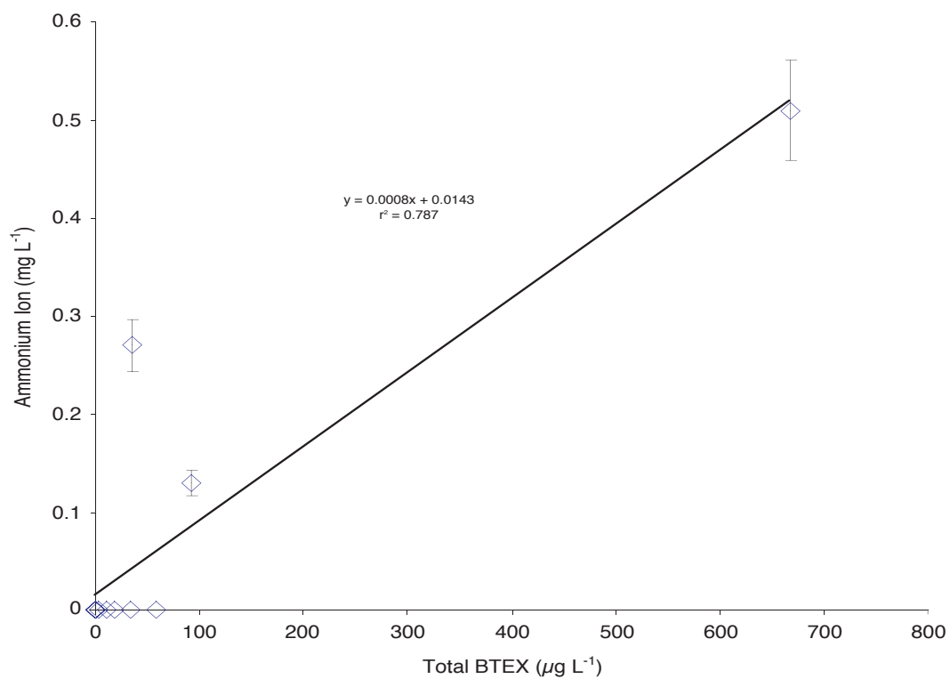
Fig. 16 — \text{NH}_4^+ concentrations related to total BTEX over sampling area
