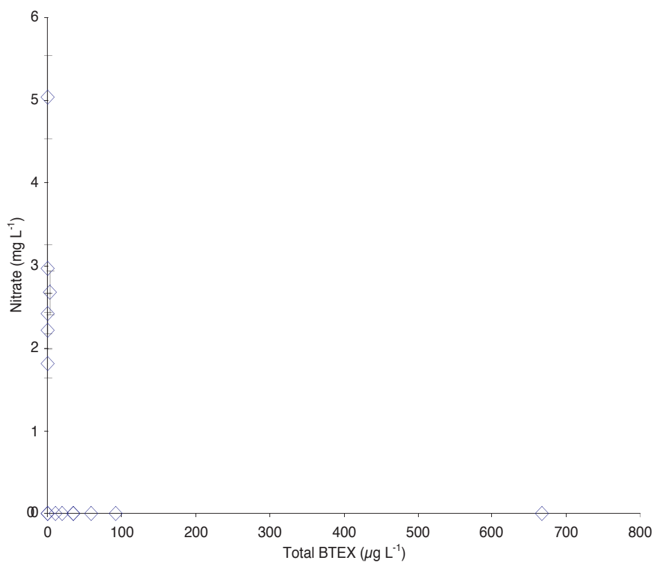
Fig. 17 — \text{NO}_3^- concentrations related to total BTEX over sampling area
