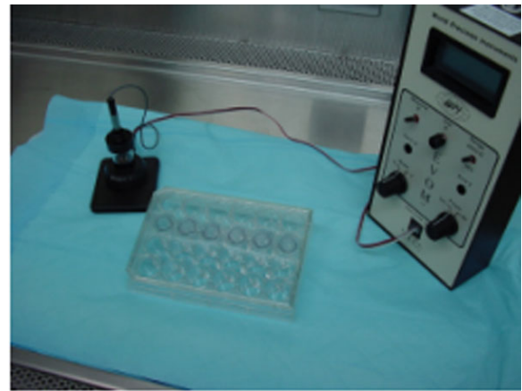
Figure 2. Measurement of transendothelial electrical resistance. (A) In the in vitro vascular leak model, human primary endothelial cells (HUVEC) were grown to confluency on the surface of a cell environment insert immersed in cell growth medium in a 24-well plate. Confluency of the cell monolayer was determined by measuring the transendothelial electrical resistance (TEER) every other day, placing the insert containing the cell in a electrical chamber containing cell growth medium. (B) The chamber had one electrode on each side of the insert. An electric current was passed through the insert and the electrical resistance was measured by the Endohm voltmeter.
