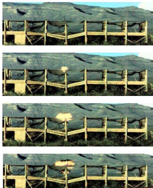
Fig. 5. Mortar pre-detonation sequence
