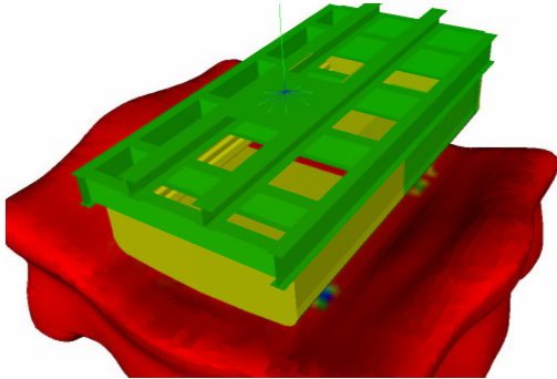
Figure 5. Mine Blast Interacting with Vehicle Hull
