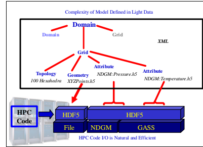
Figure 1. XDMF.
