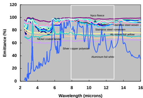
Figure 4. Emittance data collected for fabrics, metal fabrics, and foils
